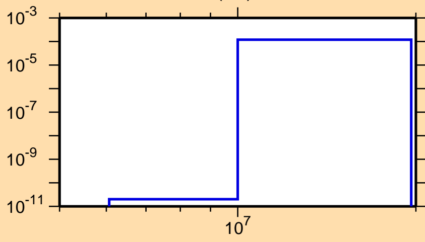
\sigma vs. E for ^{195}\text{Pb}(n,t)
