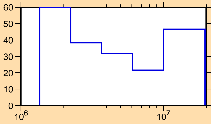
\Delta\sigma/\sigma vs. E for ^{195}\text{Pb}(n,n\text{cont.})
