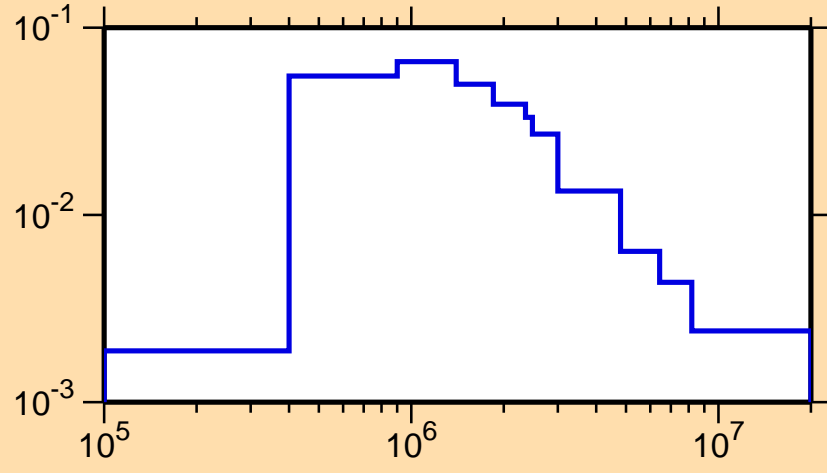
\sigma vs. E for ^{195}\text{Pb}(n,n_3)
