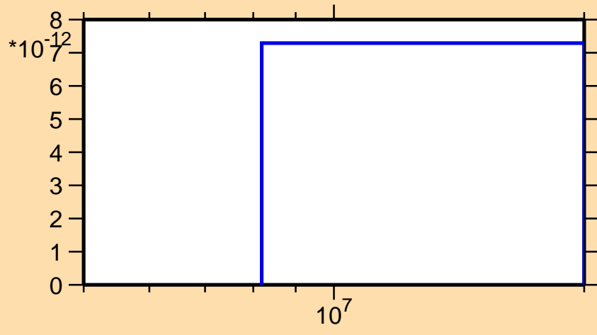
\sigma vs. E for ^{195}\text{Pb}(n,3n\alpha)
