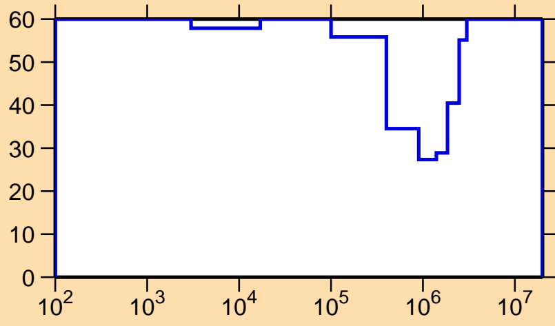
\Delta\sigma/\sigma vs. E for ^{195}\text{Pb}(n,\gamma)
