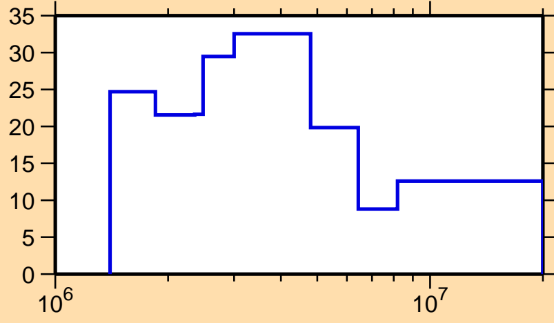
\Delta\sigma/\sigma vs. E for ^{195}\text{Pb}(n, tot.)
