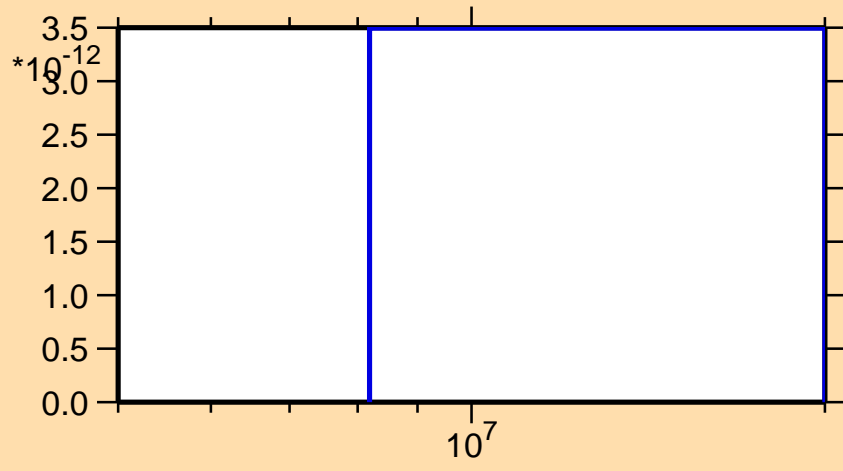
\sigma vs. E for ^{195}\text{Pb}(n,3n\alpha)
