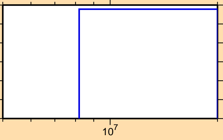
\sigma vs. E for ^{195}\text{Pb}(n,2n\alpha)
