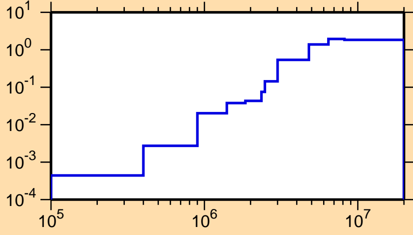
\sigma vs. E for ^{195}\text{Pb}(n,\text{inel.})
