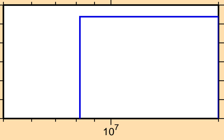
\sigma vs. E for ^{195}\text{Pb}(n,\text{nd})
