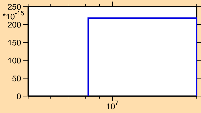
\sigma vs. E for ^{195}\text{Pb}(n,nt)
