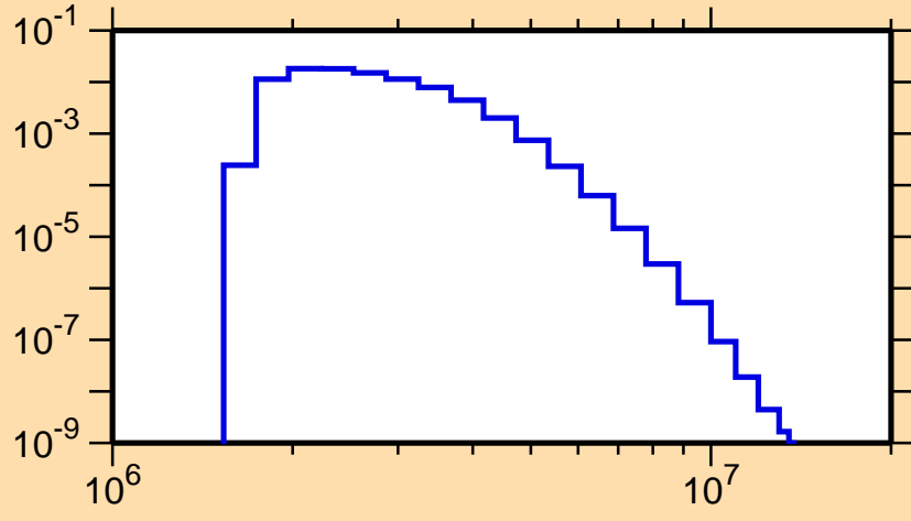
\sigma vs. E for ^{196}\text{Pb}(n,n_4)
