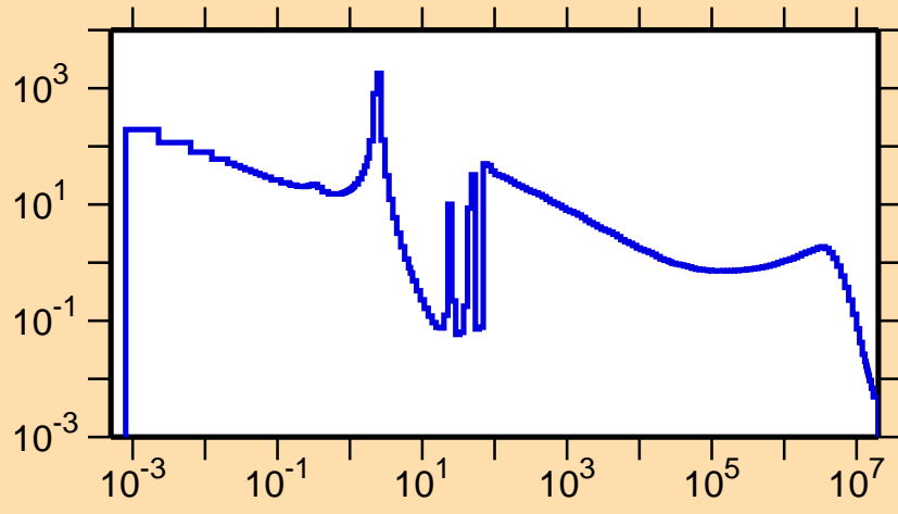
\sigma vs. E for ^{196}\text{Pb}(n,\gamma)
