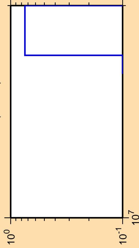
\Delta\sigma/\sigma vs. E for ^{196}\text{Pb} (mt 34)
