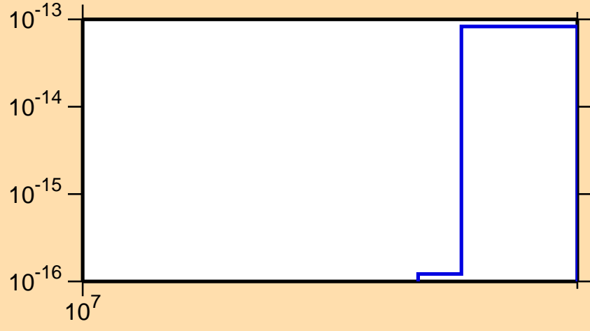
\sigma vs. E for ^{196}\text{Pb} (mt 34)
