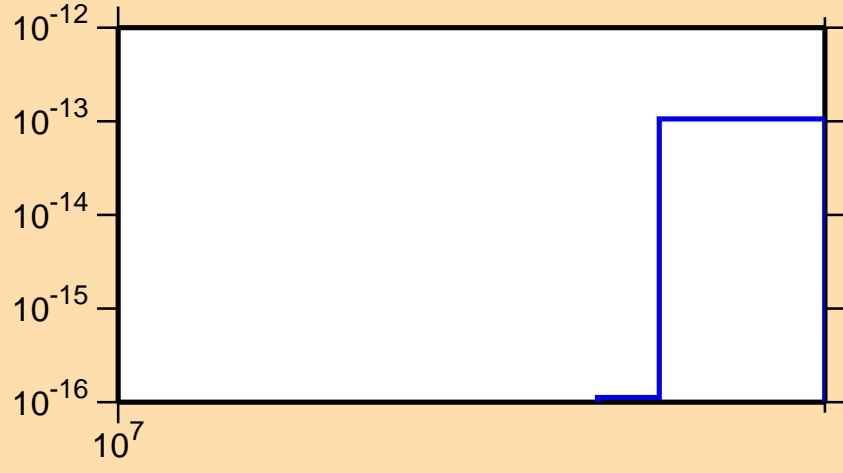
\sigma vs. E for ^{196}\text{Pb}(n,\text{pt})
