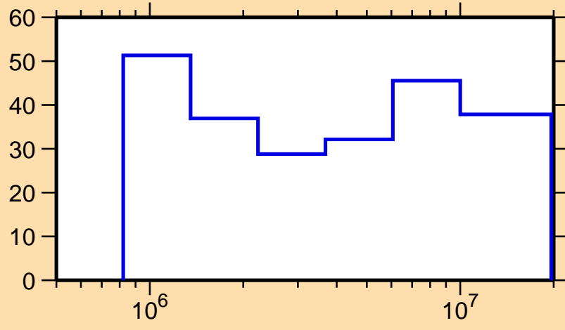
\Delta\sigma/\sigma vs. E for ^{196}\text{Pb}(n,\text{el.})
