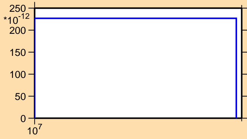
\sigma vs. E for ^{196}\text{Pb}(n,\text{nd})
