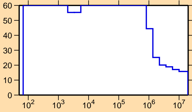
\Delta\sigma/\sigma vs. E for ^{196}\text{Pb}(n,\text{nonel.})
