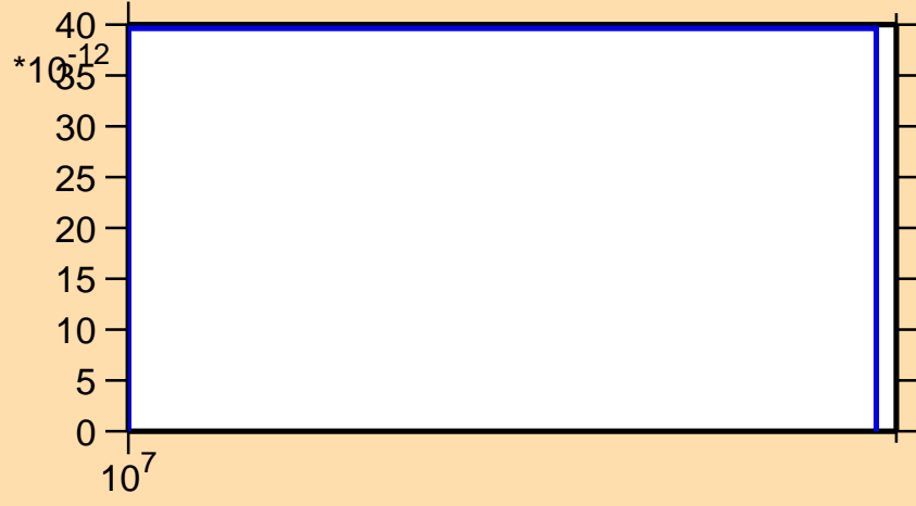
\sigma vs. E for ^{196}\text{Pb}(\text{mt } 45)
