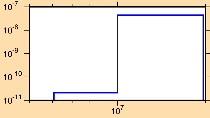
\sigma vs. E for ^{196}\text{Pb}(n,p\alpha)
