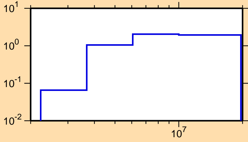
\sigma vs. E for ^{196}\text{Pb}(n,n\text{cont.})
