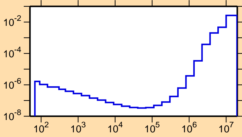
\sigma vs. E for ^{196}\text{Pb}(n,p)
