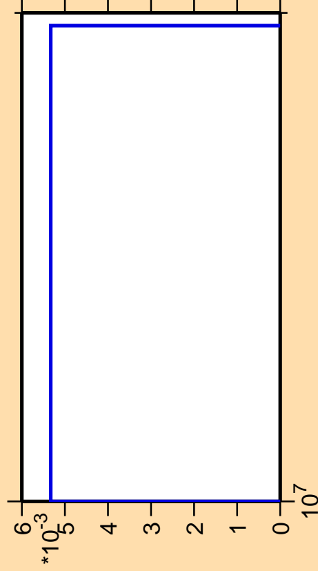
\Delta\sigma/\sigma vs. E for ^{196}\text{Pb}(\text{mt } 34)
