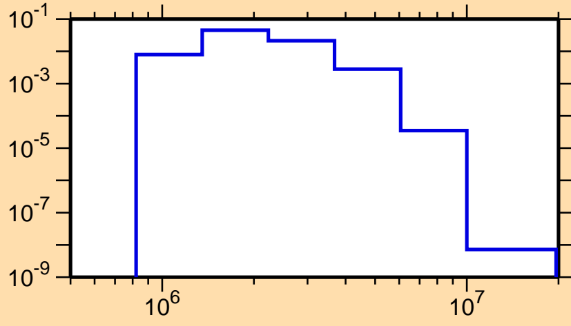
\sigma vs. E for ^{196}\text{Pb}(n,n_2)
