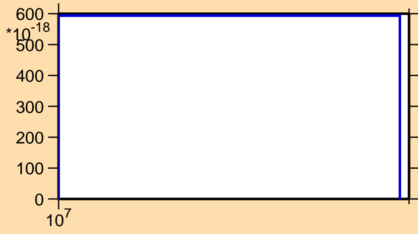
\sigma vs. E for ^{196}\text{Pb}(\text{mt } 34)
