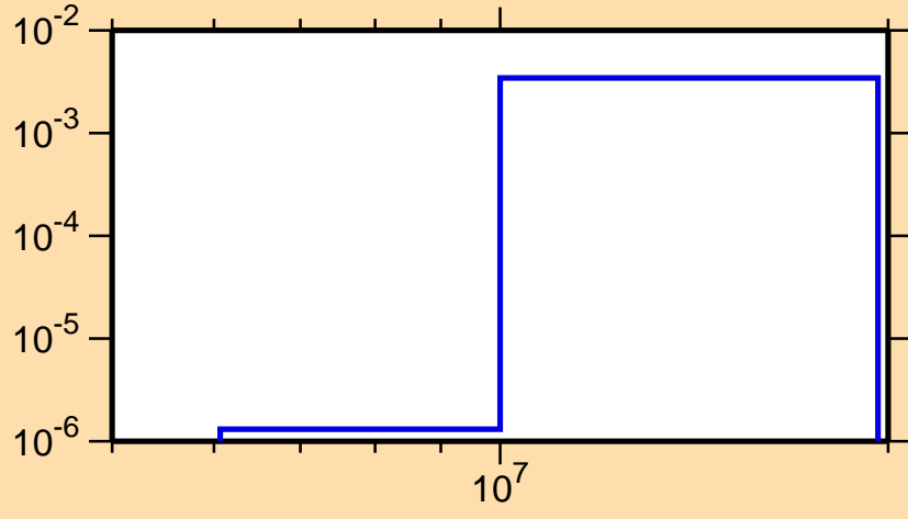
\sigma vs. E for ^{196}\text{Pb}(n,np)
