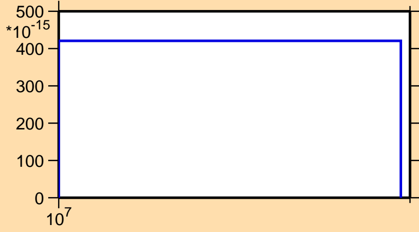
\sigma vs. E for ^{196}\text{Pb}(n,nt)
