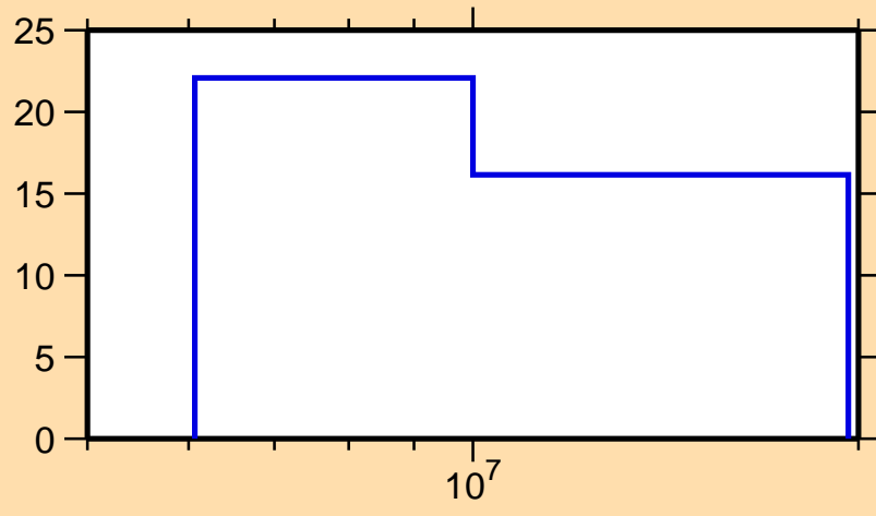
\Delta\sigma/\sigma vs. E for ^{196}\text{Pb}(n,\text{tot.})
