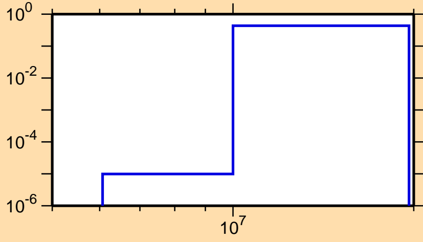
\sigma vs. E for ^{196}\text{Pb}(n,2n)
