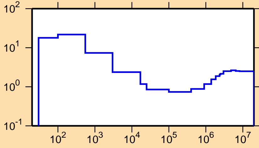
\sigma vs. E for ^{196}\text{Pb}(n,\text{nonel.})
