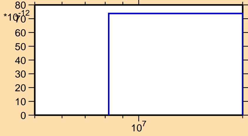
\sigma vs. E for ^{196}\text{Pb}(n,3n\alpha)
