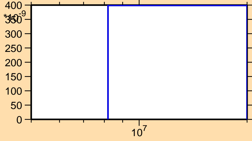
\sigma vs. E for ^{196}\text{Pb}(n,2n\alpha)
