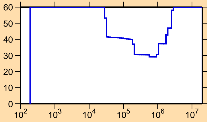
\Delta\sigma/\sigma vs. E for ^{197}\text{Pb}(n,\gamma)
