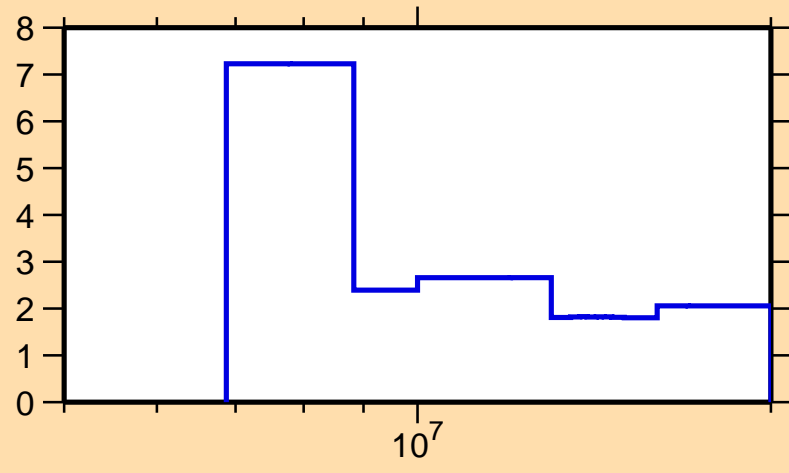
\Delta\sigma/\sigma vs. E for ^{197}\text{Pb}(n,\text{tot.})
