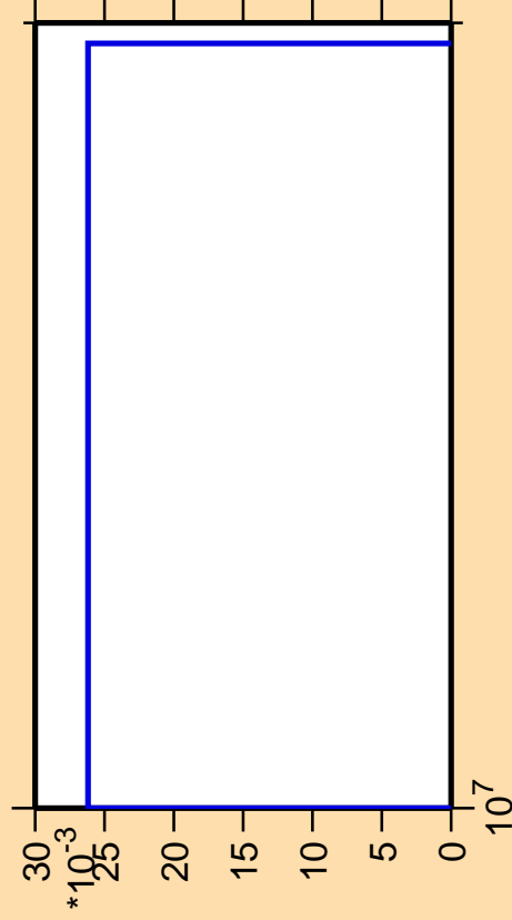
\Delta\sigma/\sigma vs. E for ^{197}\text{Pb}(n,3n\alpha)
