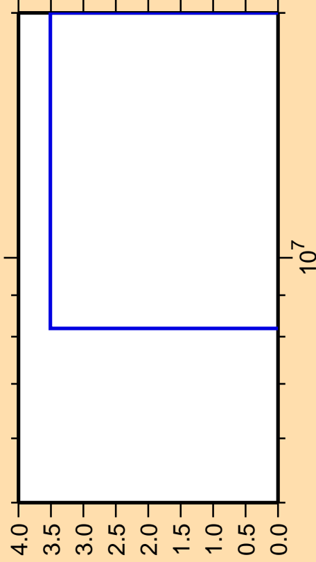
\Delta\sigma/\sigma vs. E for ^{197}\text{Pb}(n,pd)
