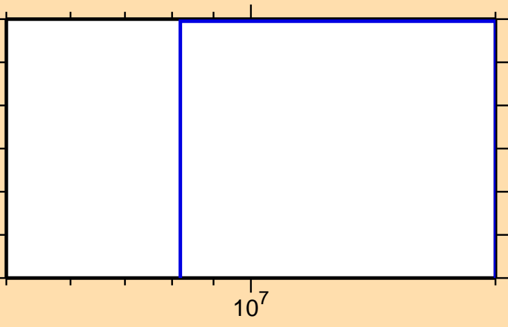
\sigma vs. E for ^{197}\text{Pb}(n,2n\alpha)
