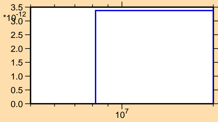
\sigma vs. E for ^{197}\text{Pb}(\text{mt } 45)
