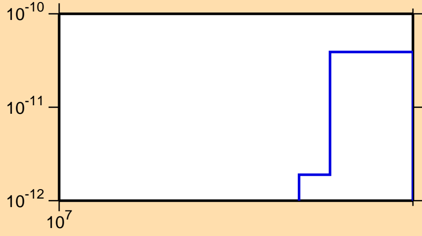
\sigma vs. E for ^{197}\text{Pb}(n,\text{pd})
