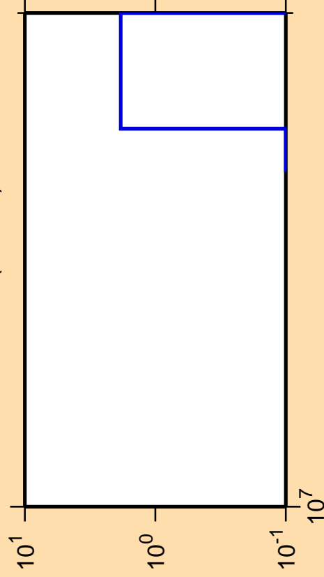
\Delta\sigma/\sigma vs. E for ^{197}\text{Pb}(n,3n\alpha)
