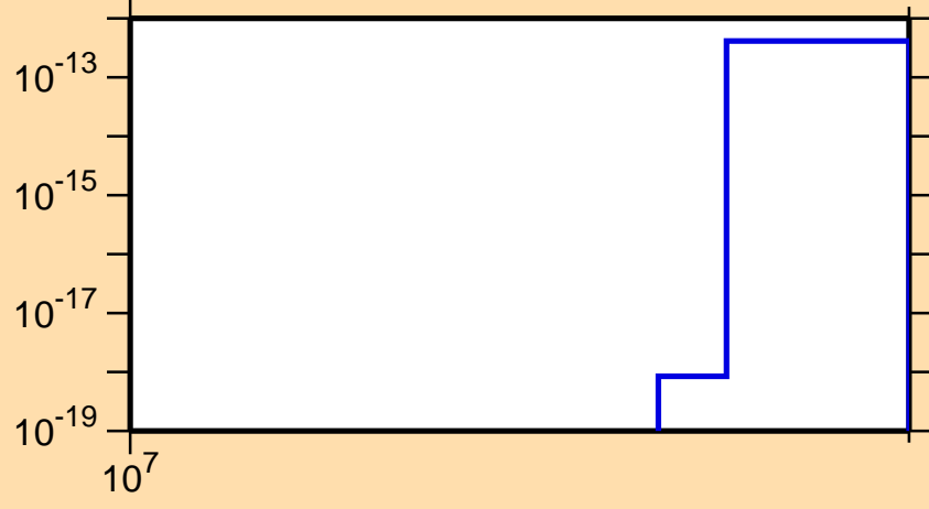
\sigma vs. E for ^{197}\text{Pb}(n,3n\alpha)
