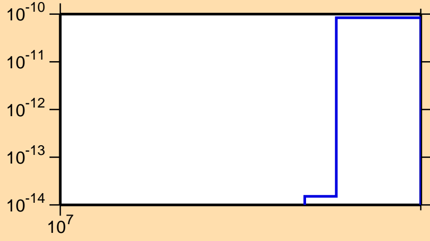
\sigma vs. E for ^{197}\text{Pb}(n,nt)
