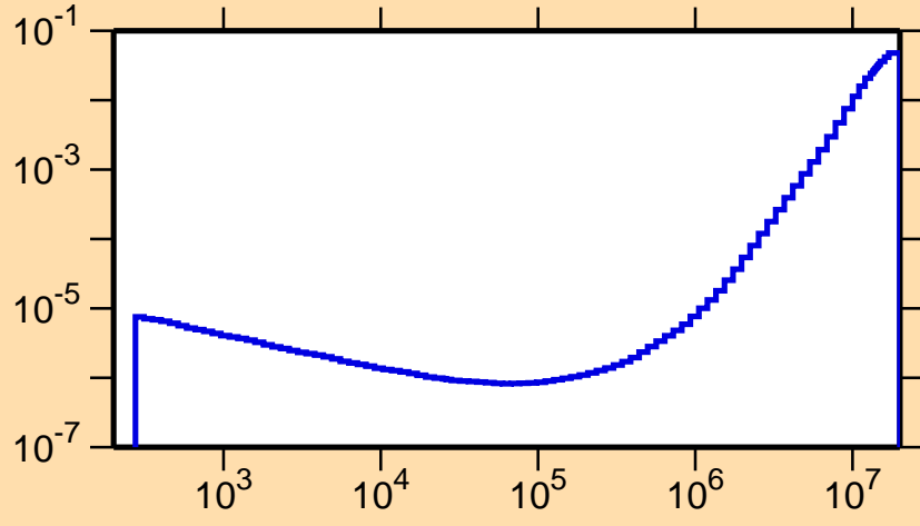
\sigma vs. E for ^{197}\text{Pb}(n,p)
