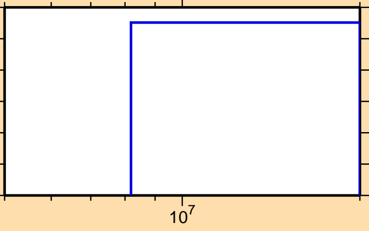
\sigma vs. E for ^{197}\text{Pb}(n,3n)
