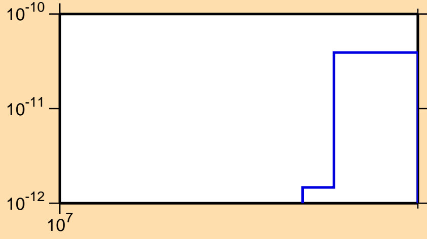
\sigma vs. E for ^{198}\text{Pb}(n,\text{pd})
