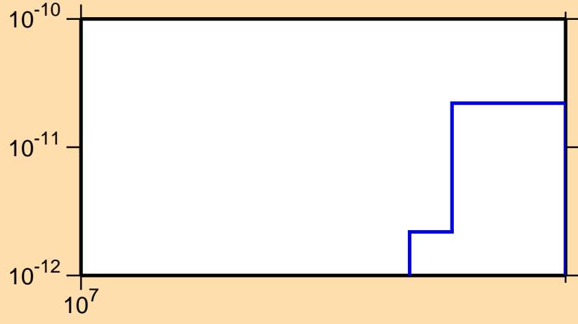
\sigma vs. E for ^{198}\text{Pb}(\text{mt117})
