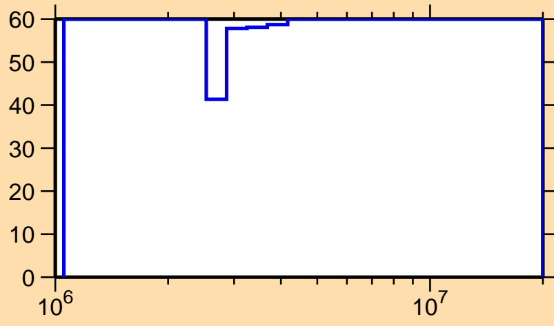
\Delta\sigma/\sigma vs. E for ^{198}\text{Pb}(n,n_1)
