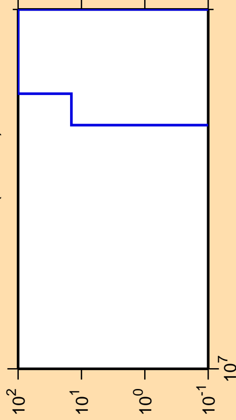
\Delta\sigma/\sigma vs. E for ^{198}\text{Pb}(\text{mt117})
