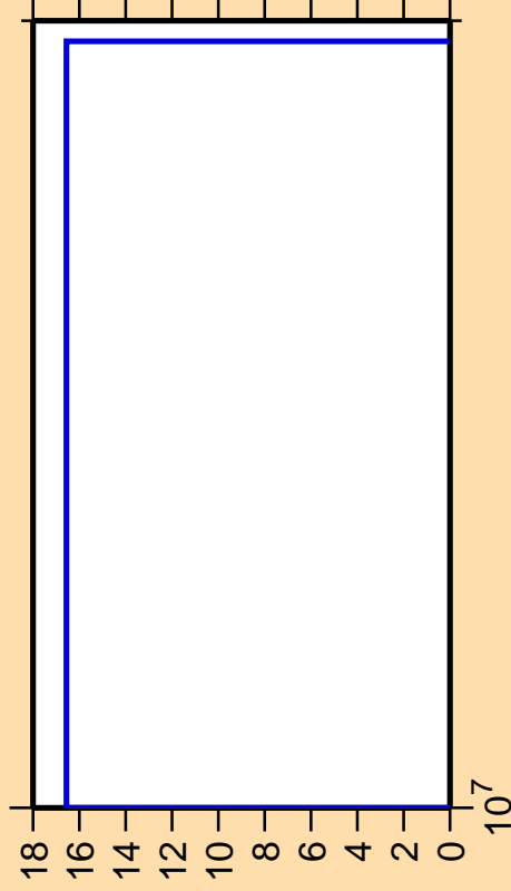
\Delta\sigma/\sigma vs. E for ^{198}\text{Pb} (mt 45)
