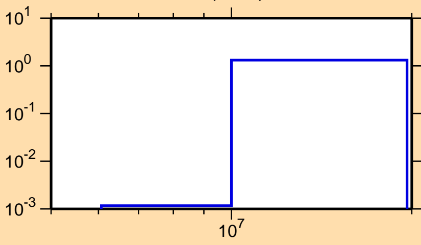
\sigma vs. E for ^{198}\text{Pb}(n,2n)
