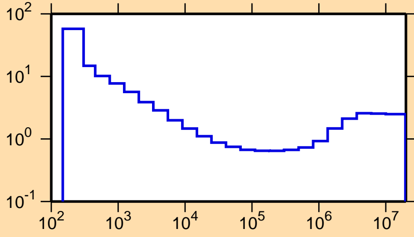
\sigma vs. E for ^{198}\text{Pb}(n,\text{nonel.})
