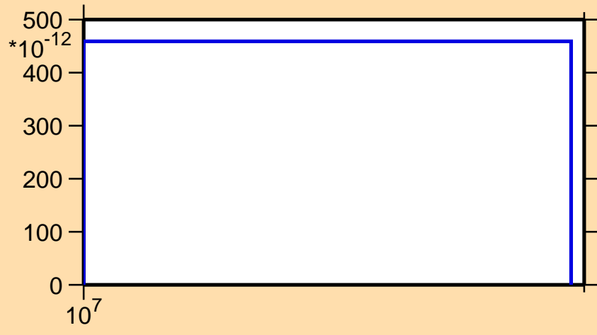
\sigma vs. E for ^{198}\text{Pb}(n,\text{nd})
