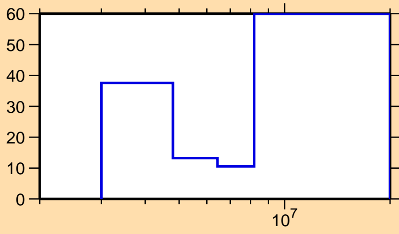
\Delta\sigma/\sigma vs. E for ^{198}\text{Pb}(n,n\text{cont.})
