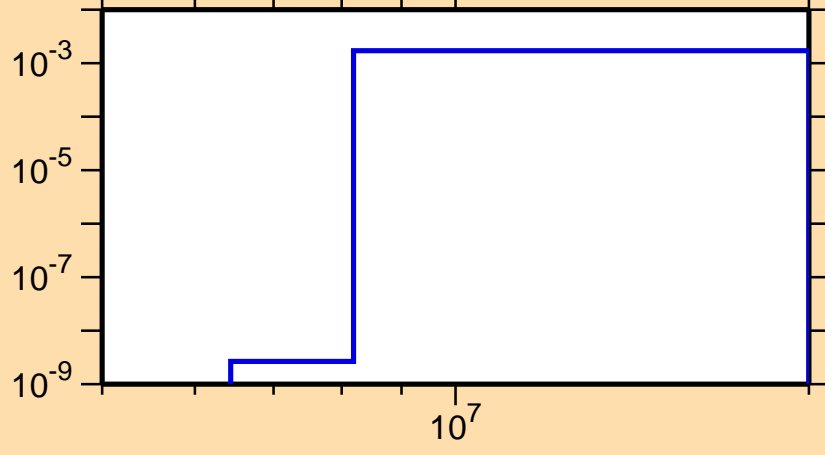
\sigma vs. E for ^{198}\text{Pb}(n,np)
