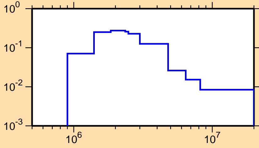
\sigma vs. E for ^{198}\text{Pb}(n,n_1)
