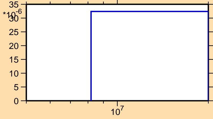
\sigma vs. E for ^{198}\text{Pb}(n,3n)
