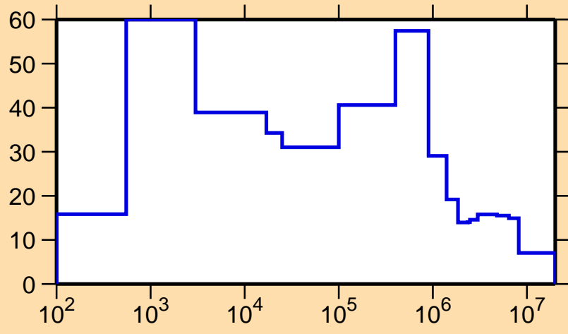
\Delta\sigma/\sigma vs. E for ^{198}\text{Pb}(n,\text{tot.})
