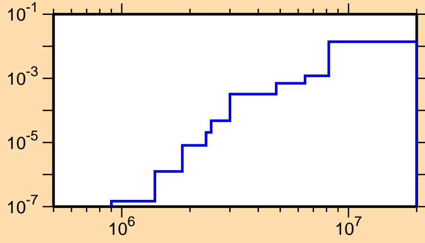
\sigma vs. E for ^{198}\text{Pb}(n,p)
