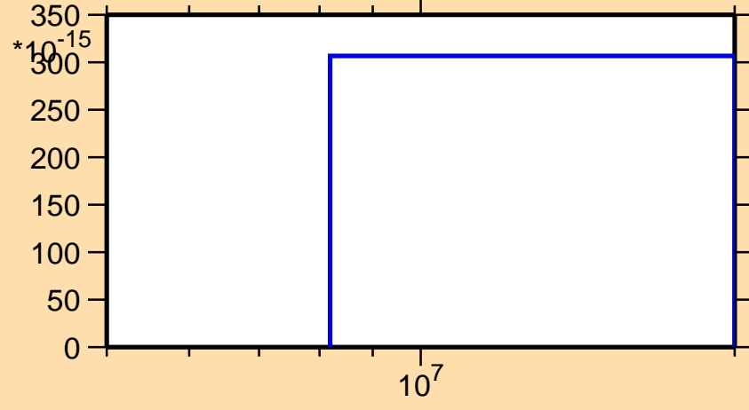
\sigma vs. E for ^{198}\text{Pb}(\text{mt117})
