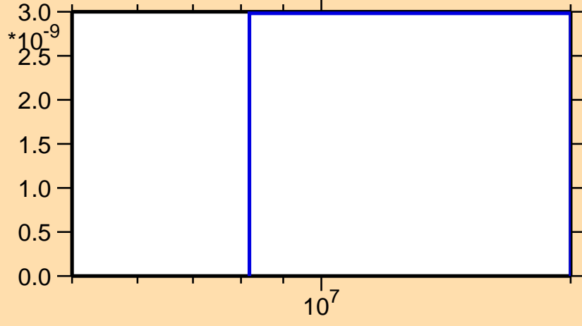
\sigma vs. E for ^{198}\text{Pb}(n,p\alpha)
