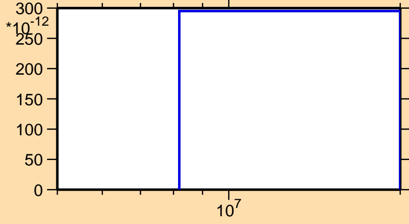
\sigma vs. E for ^{198}\text{Pb}(n,3n\alpha)
