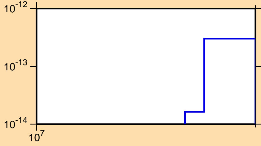
\sigma vs. E for ^{200}\text{Pb}(\text{mt117})
