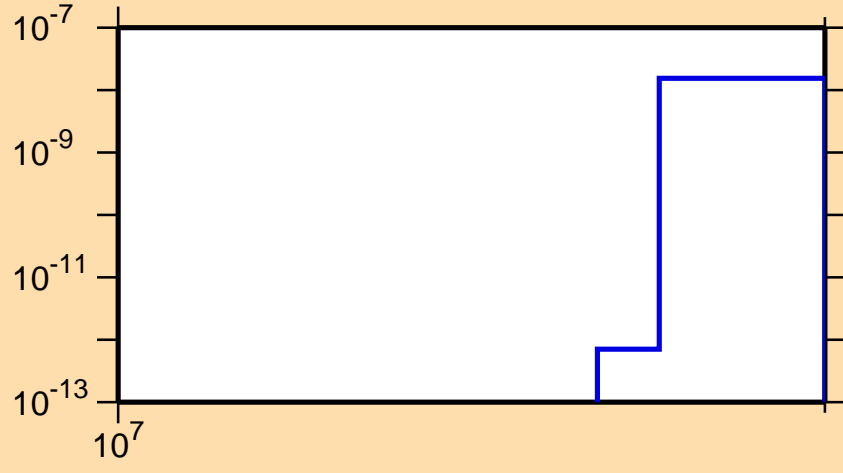
\sigma vs. E for ^{200}\text{Pb}(n,2np)
