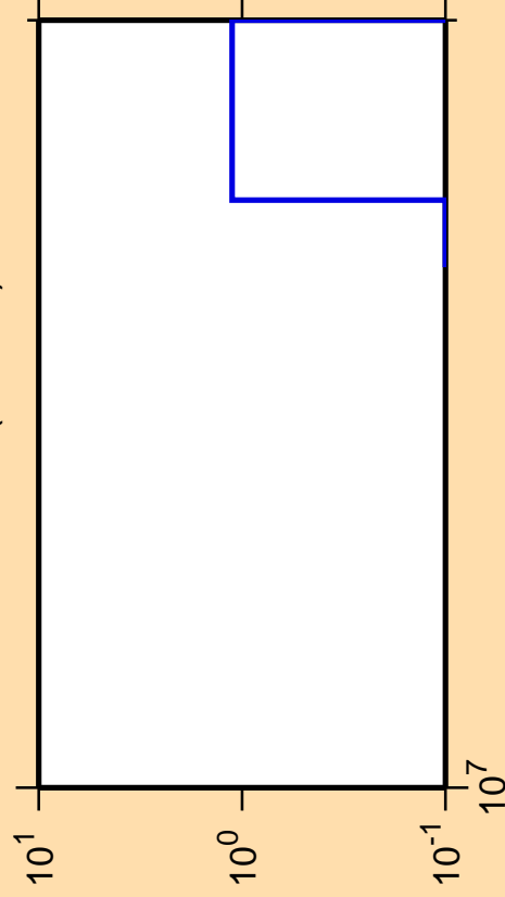
\Delta\sigma/\sigma vs. E for ^{200}\text{Pb}(\text{mt117})
