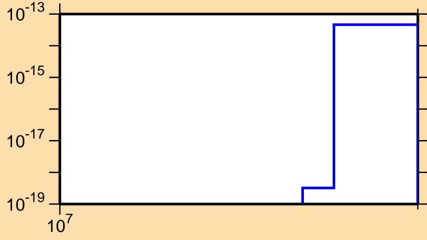
\sigma vs. E for ^{200}\text{Pb}(n,3n\alpha)
