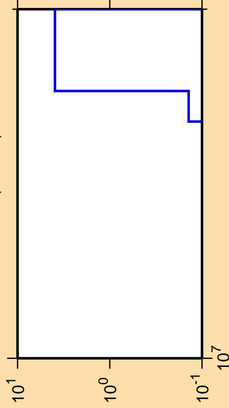
\Delta\sigma/\sigma vs. E for ^{200}\text{Pb} (mt 45)
