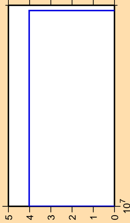
\Delta\sigma/\sigma vs. E for ^{200}\text{Pb}(n,nt)
