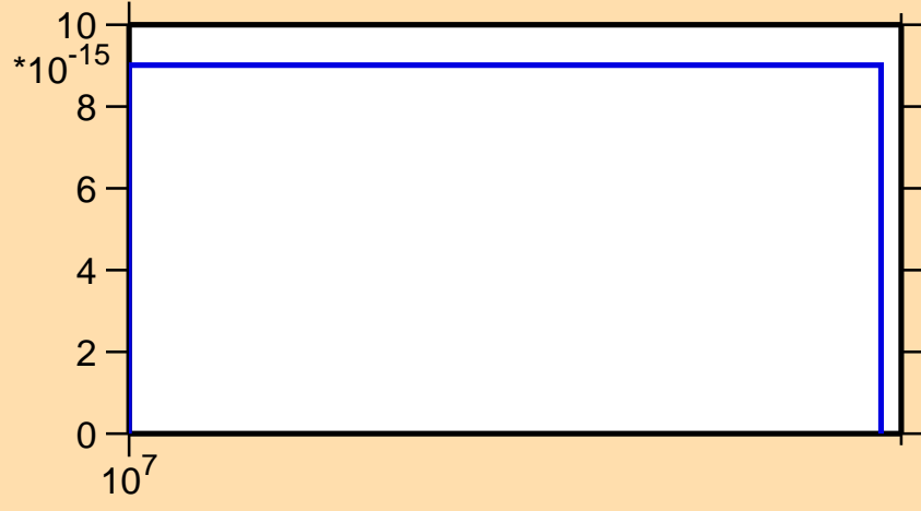
\sigma vs. E for ^{200}\text{Pb} (mt 45)
