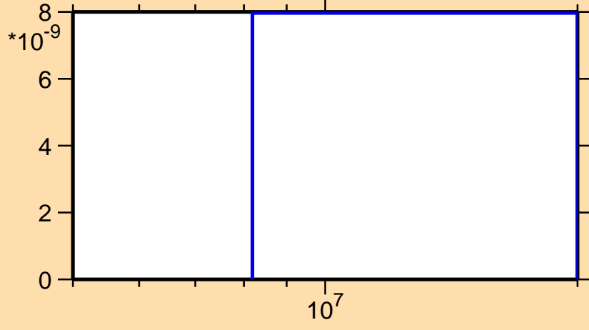
\sigma vs. E for ^{200}\text{Pb}(n,2n\alpha)
