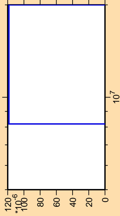
\Delta\sigma/\sigma vs. E for ^{200}\text{Pb}(n,3n\alpha)
