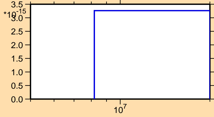
\sigma vs. E for ^{200}\text{Pb}(\text{mt117})
