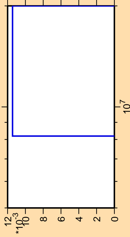
\Delta\sigma/\sigma vs. E for ^{200}\text{Pb}(\text{mt117})
