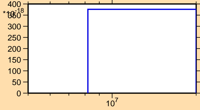
\sigma vs. E for ^{200}\text{Pb}(n,3n\alpha)
