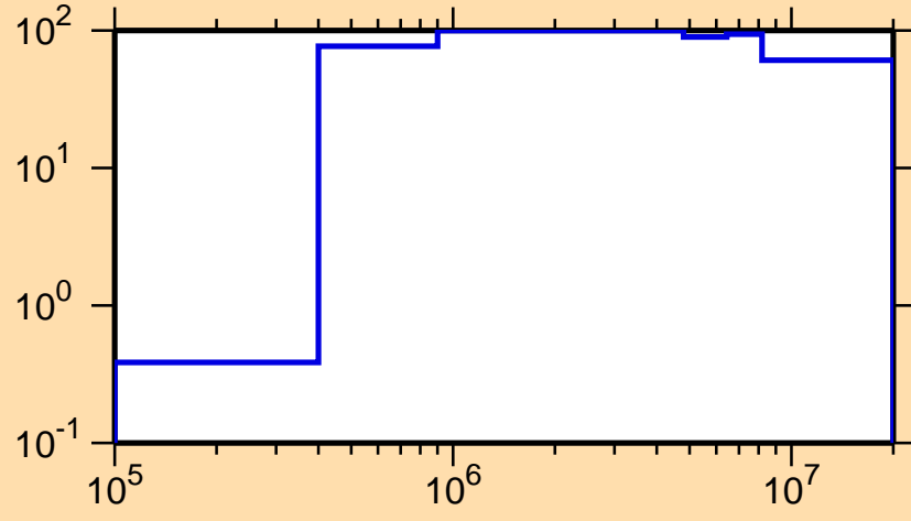
\Delta\sigma/\sigma vs. E for ^{200}\text{Pb}(n,p)
