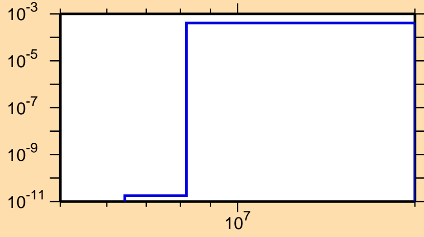
\sigma vs. E for ^{200}\text{Pb}(n,d)
