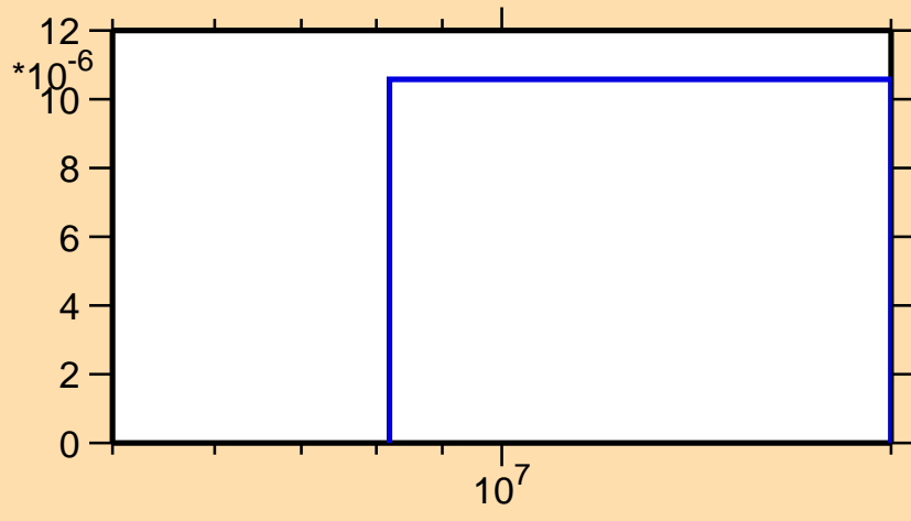
\sigma vs. E for ^{200}\text{Pb}(n,t)
