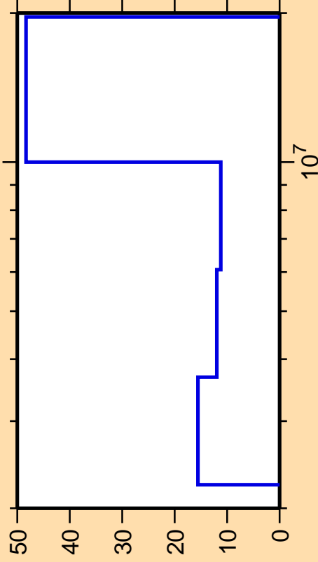
\Delta\sigma/\sigma vs. E for ^{201}\text{Pb}(n,n\text{cont.})
