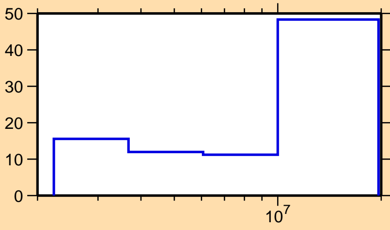
\Delta\sigma/\sigma vs. E for ^{201}\text{Pb}(n,n\text{cont.})
