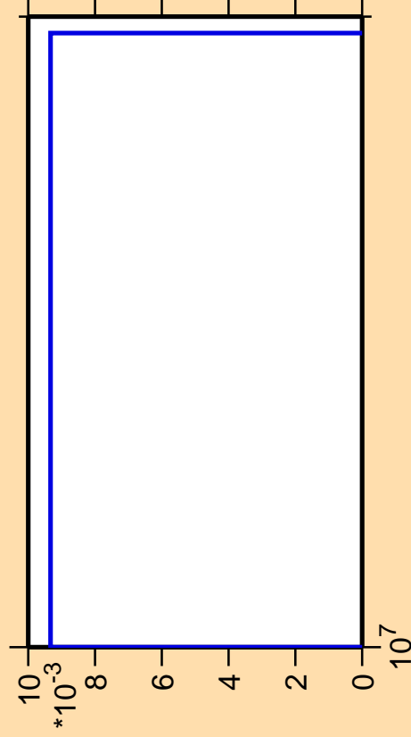
\Delta\sigma/\sigma vs. E for ^{201}\text{Pb} (mt 45)
