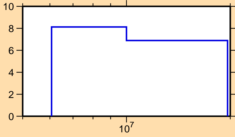
\Delta\sigma/\sigma vs. E for ^{201}\text{Pb}(n,\text{nonel.})
