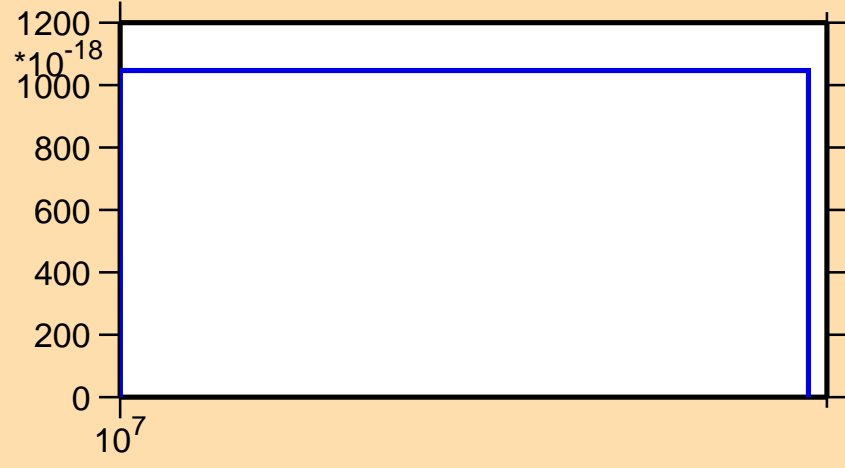
\sigma vs. E for ^{201}\text{Pb} (mt 45)
