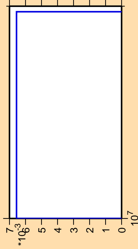
\Delta\sigma/\sigma vs. E for ^{201}\text{Pb}(n,pd)
