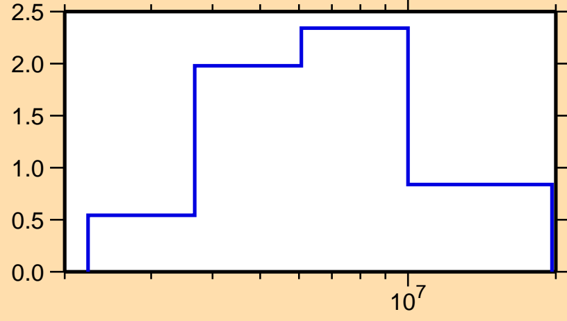
\sigma vs. E for ^{201}\text{Pb}(n,n\text{cont.})
