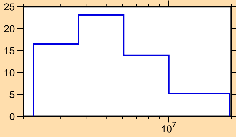
\Delta\sigma/\sigma vs. E for ^{201}\text{Pb}(n,\text{el.})
