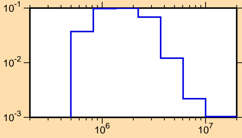
\sigma vs. E for ^{201}\text{Pb}(n,n_3)
