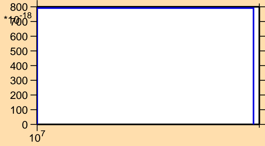
\sigma vs. E for ^{201}\text{Pb}(n,pd)
