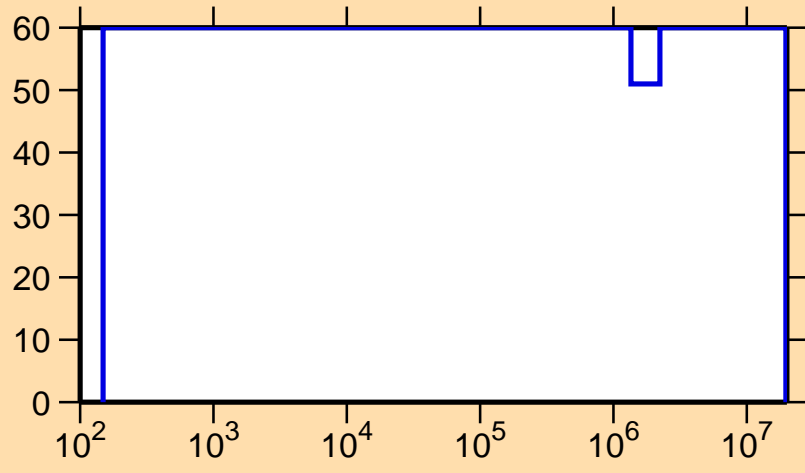
\Delta\sigma/\sigma vs. E for ^{201}\text{Pb}(n,p)
