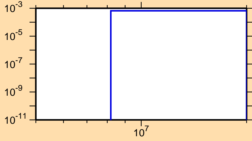
\sigma vs. E for ^{201}\text{Pb}(n,np)
