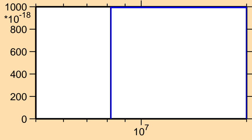
\sigma vs. E for ^{201}\text{Pb}(\text{mt } 45)
