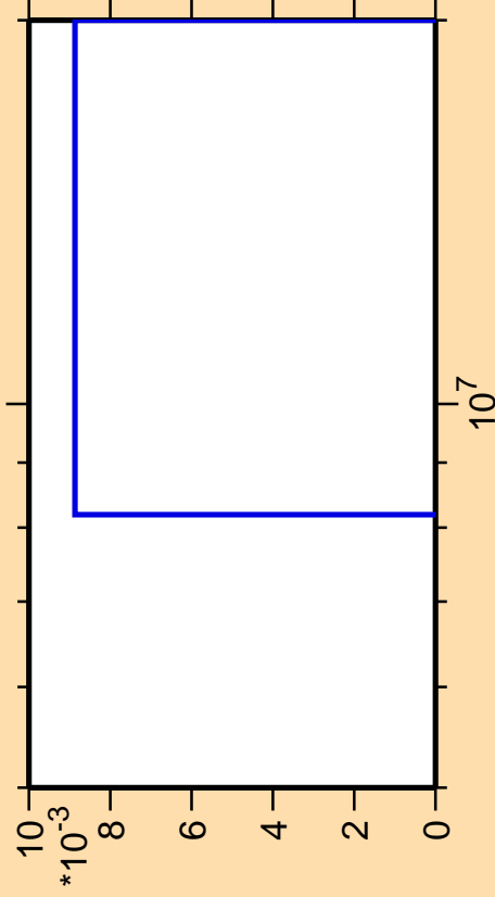
\Delta\sigma/\sigma vs. E for ^{201}\text{Pb}(\text{mt } 45)
