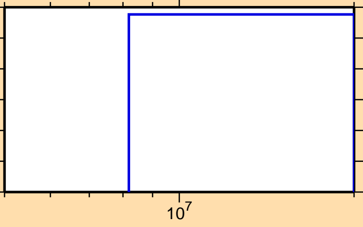
\sigma vs. E for ^{201}\text{Pb}(n,3n)
