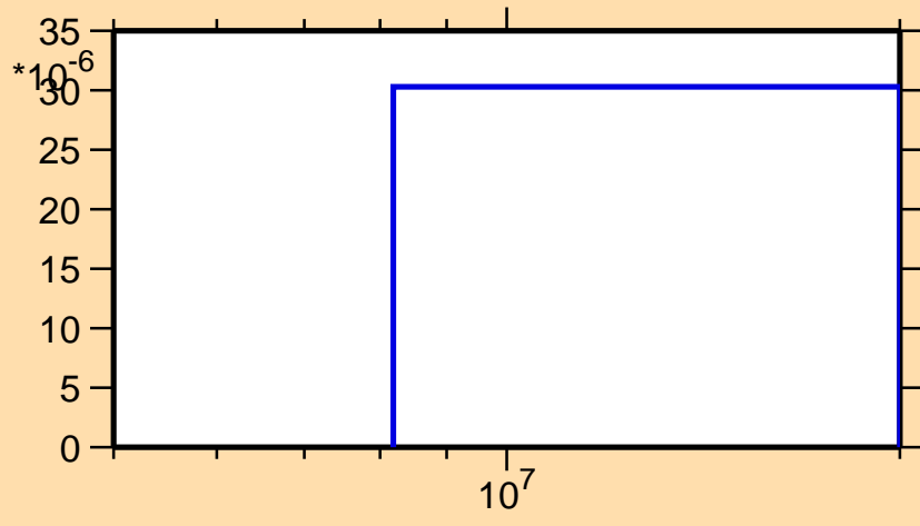
\sigma vs. E for ^{201}\text{Pb}(n,t)
