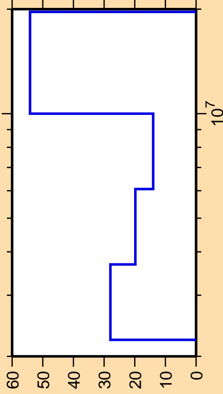
\Delta\sigma/\sigma vs. E for ^{202}\text{Pb}(n,n\text{cont.})
