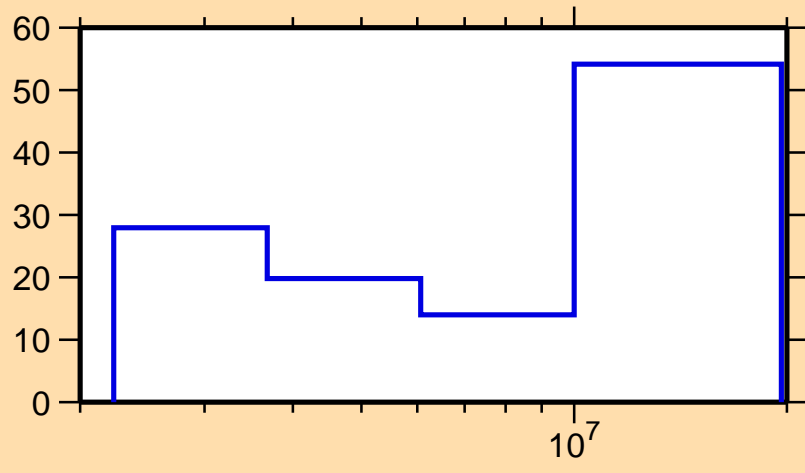
\Delta\sigma/\sigma vs. E for ^{202}\text{Pb}(n,n\text{cont.})
