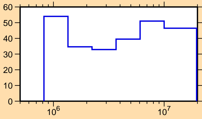
\Delta\sigma/\sigma vs. E for ^{202}\text{Pb}(n,n_1)
