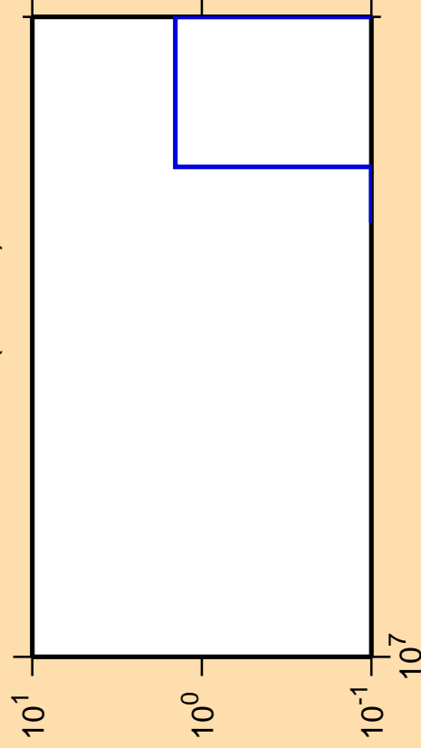
\Delta\sigma/\sigma vs. E for ^{202}\text{Pb}(n,3n\alpha)
