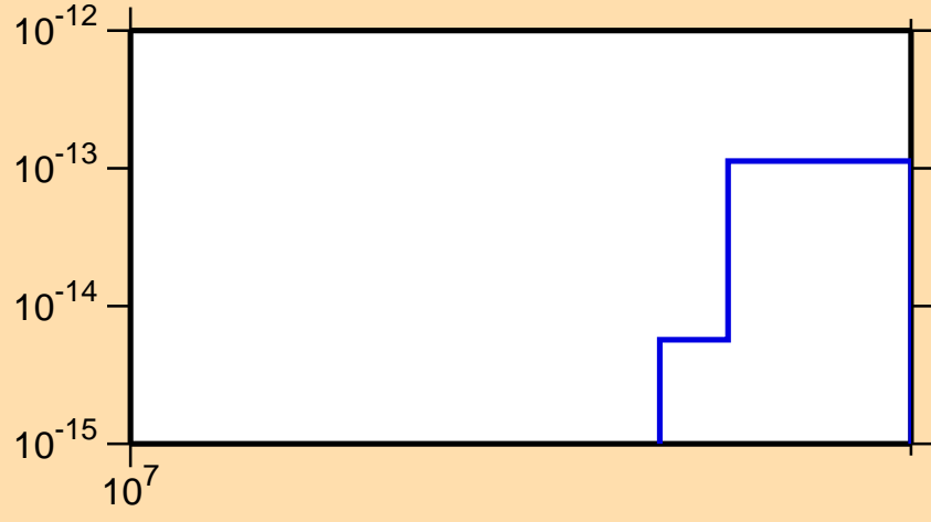
\sigma vs. E for ^{202}\text{Pb} (mt 45)
