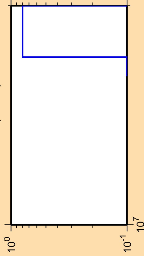
\Delta\sigma/\sigma vs. E for ^{202}\text{Pb} (mt 45)
