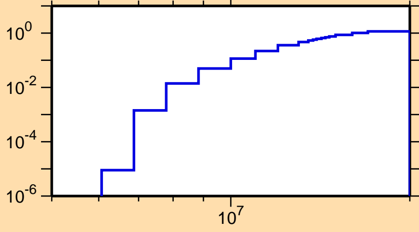
\sigma vs. E for ^{202}\text{Pb}(n,2n)
