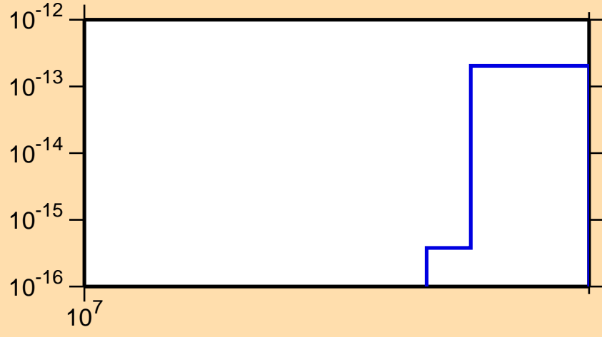
\sigma vs. E for ^{202}\text{Pb}(n,3n\alpha)
