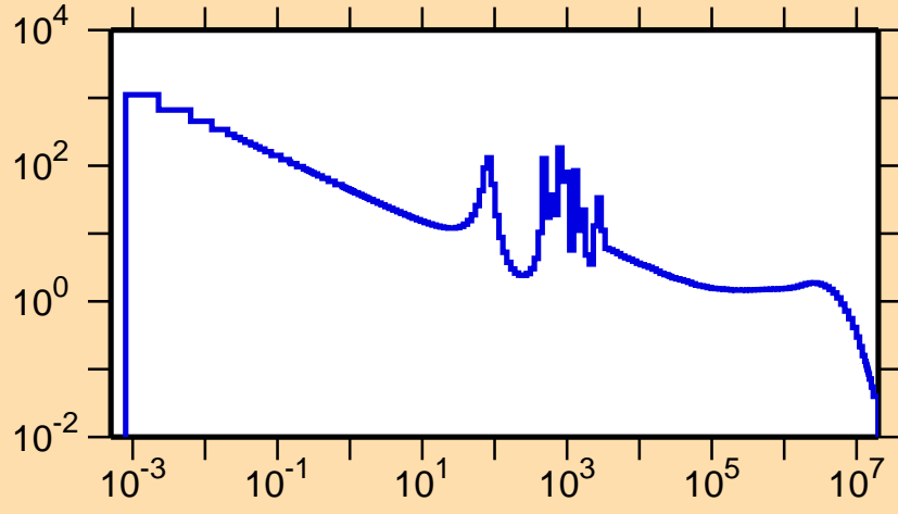
\sigma vs. E for ^{202}\text{Pb}(n,\gamma)
