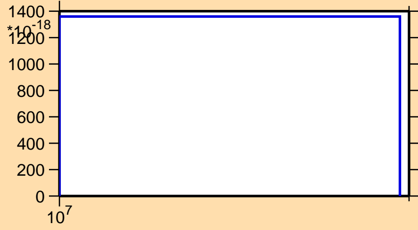
\sigma vs. E for ^{202}\text{Pb} (mt 45)
