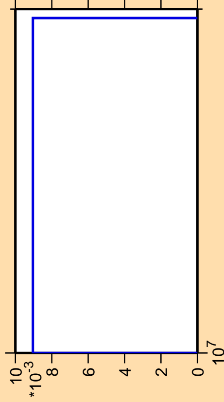
\Delta\sigma/\sigma vs. E for ^{202}\text{Pb} (mt 45)
