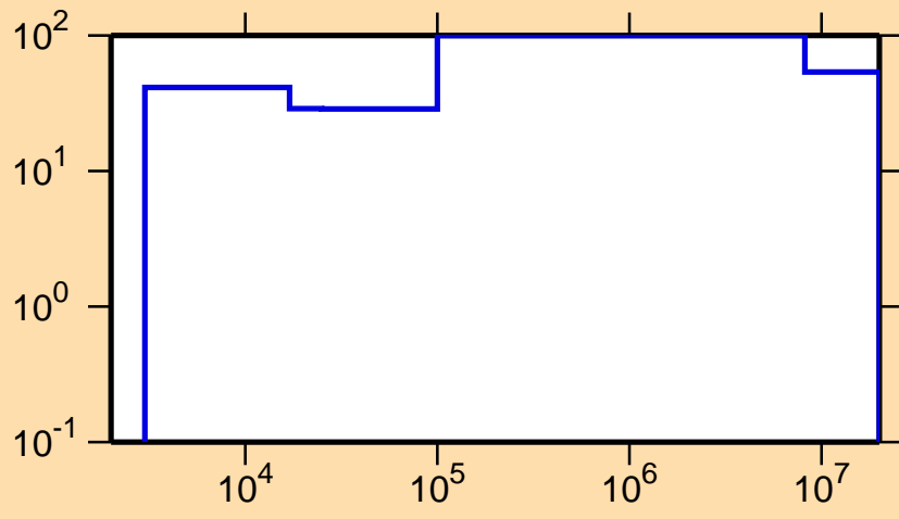
\Delta\sigma/\sigma vs. E for ^{202}\text{Pb}(n,p)
