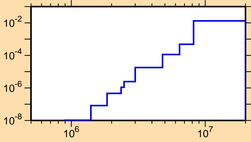
\sigma vs. E for ^{202}\text{Pb}(n,p)
