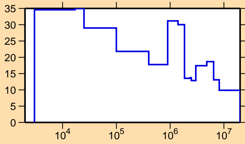
\Delta\sigma/\sigma vs. E for ^{202}\text{Pb}(n,\text{el.})
