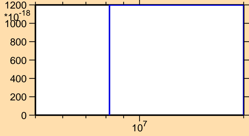
\sigma vs. E for ^{202}\text{Pb}(\text{mt } 45)
