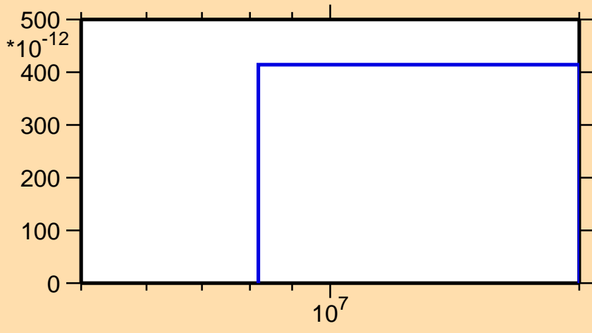
\sigma vs. E for ^{202}\text{Pb}(n,\text{He}3)
