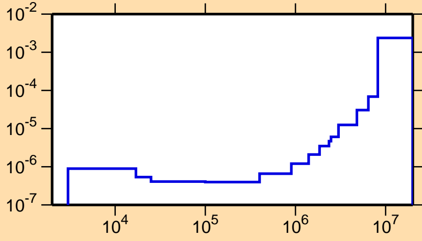
\sigma vs. E for ^{202}\text{Pb}(n,\alpha)
