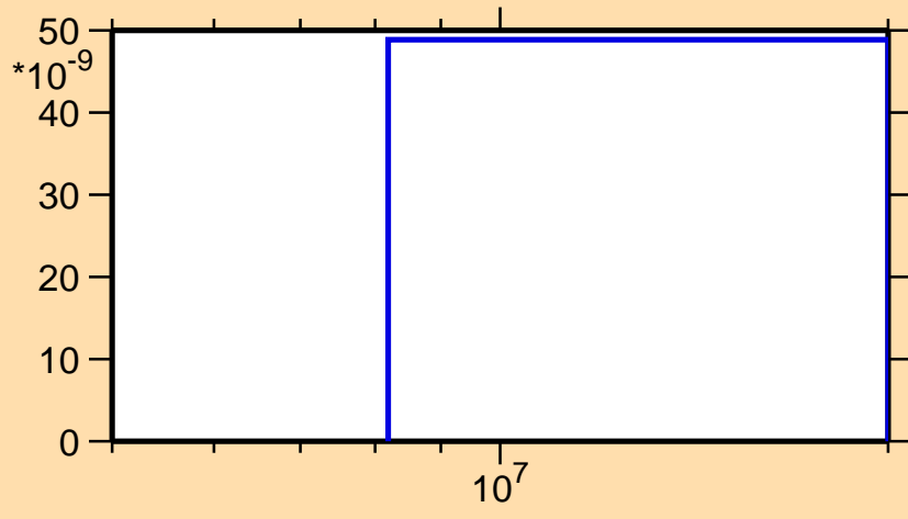
\sigma vs. E for ^{202}\text{Pb}(n,2n\alpha)
