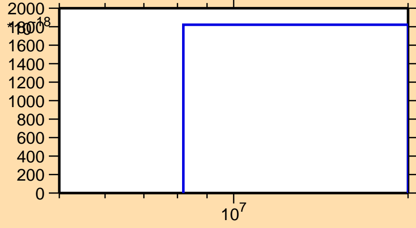
\sigma vs. E for ^{202}\text{Pb}(n,3n\alpha)
