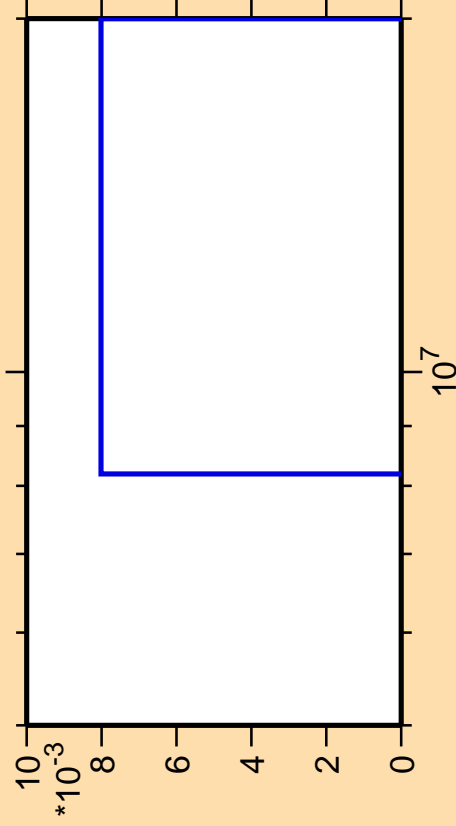
\Delta\sigma/\sigma vs. E for ^{202}\text{Pb}(\text{mt } 45)
