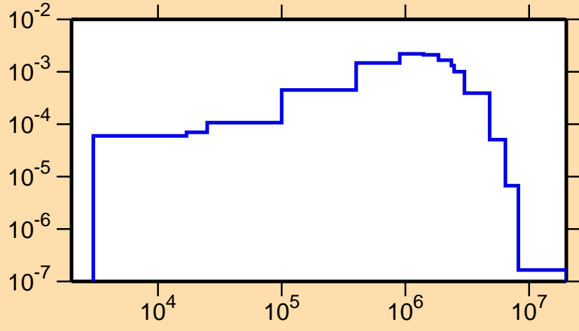
\sigma vs. E for ^{202}\text{Pb}(n,n_3)
