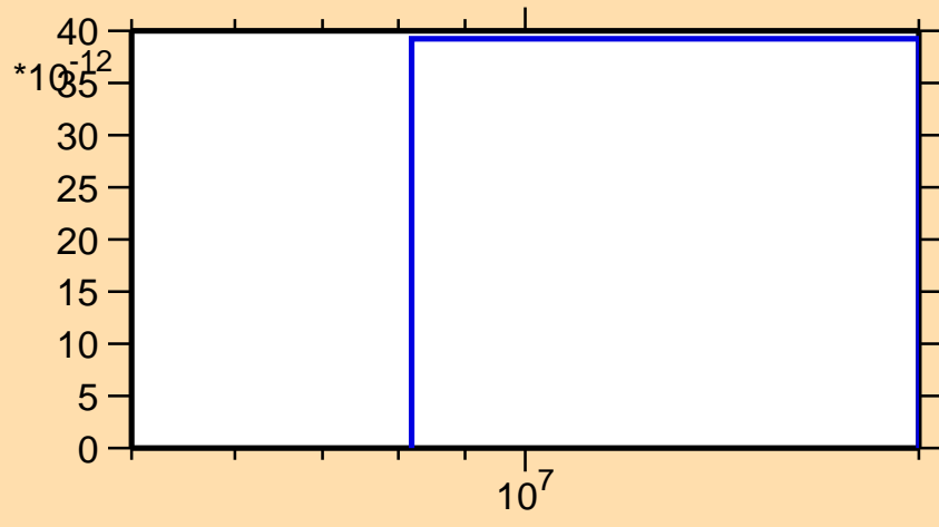
\sigma vs. E for ^{202}\text{Pb}(n,nt)
