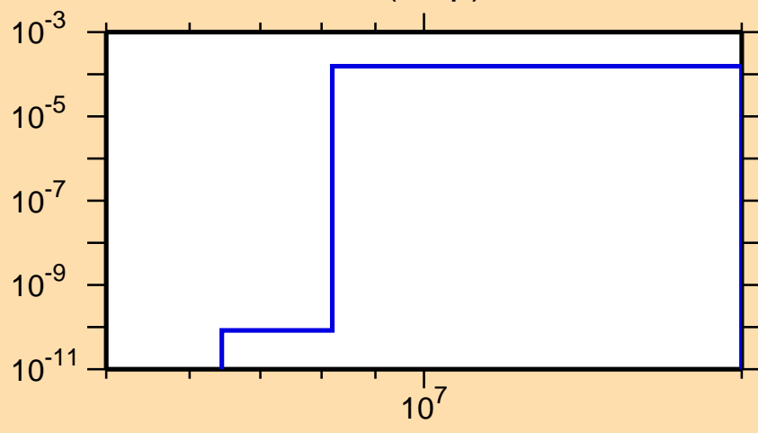
\sigma vs. E for ^{202}\text{Pb}(n,np)
