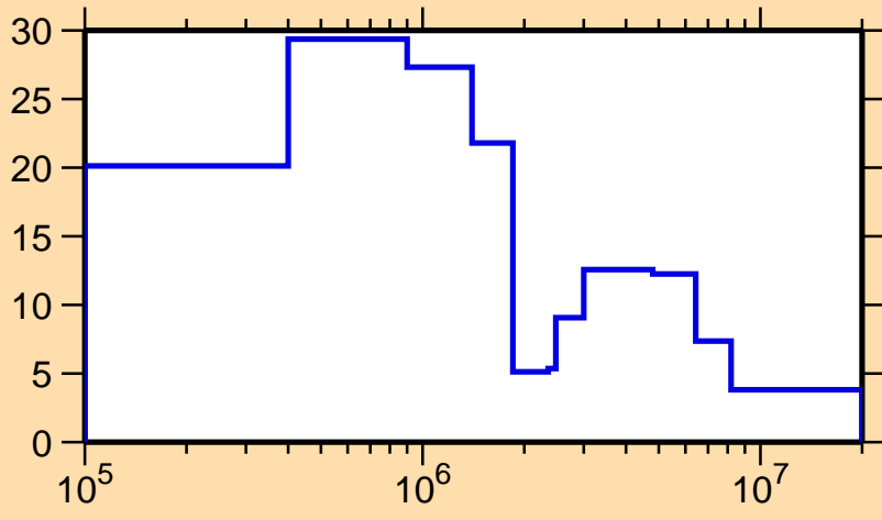
\Delta\sigma/\sigma vs. E for ^{202}\text{Pb}(n,\text{tot.})
