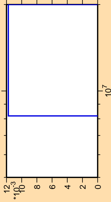
\Delta\sigma/\sigma vs. E for ^{202}\text{Pb}(n,3n\alpha)
