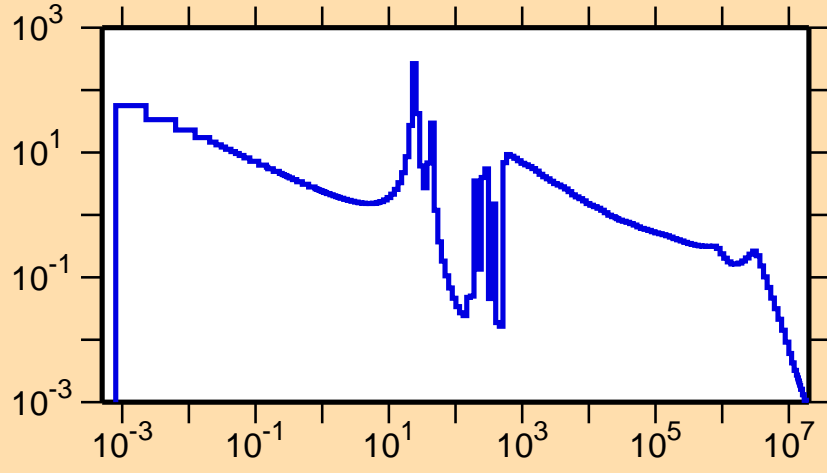
\sigma vs. E for ^{203}\text{Pb}(n,\gamma)
