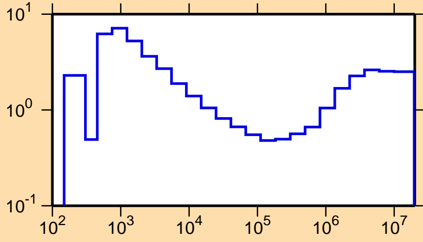
\sigma vs. E for ^{203}\text{Pb}(n,\text{nonel.})
