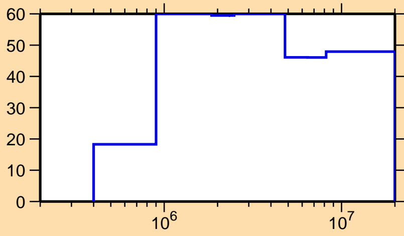
\Delta\sigma/\sigma vs. E for ^{203}\text{Pb}(n,p)
