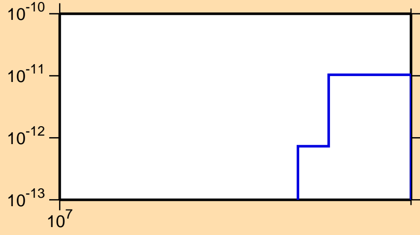
\sigma vs. E for ^{203}\text{Pb}(\text{mt } 45)
