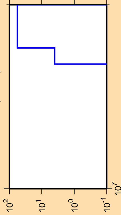
\Delta\sigma/\sigma vs. E for ^{203}\text{Pb}(\text{mt } 45)
