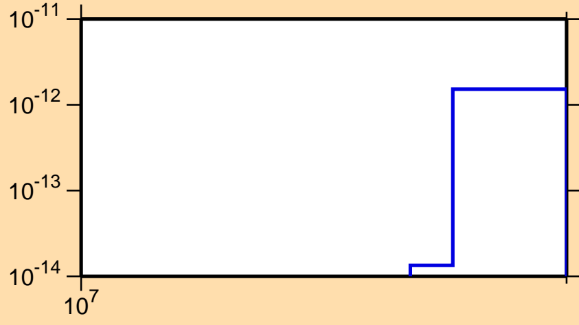
\sigma vs. E for ^{203}\text{Pb} (mt 34)
