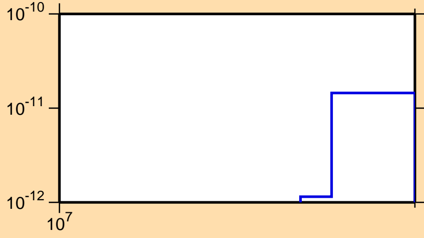
\sigma vs. E for ^{203}\text{Pb}(\text{mt117})
