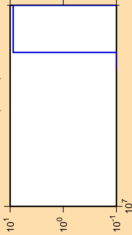
\Delta\sigma/\sigma vs. E for ^{203}\text{Pb} (mt 34)
