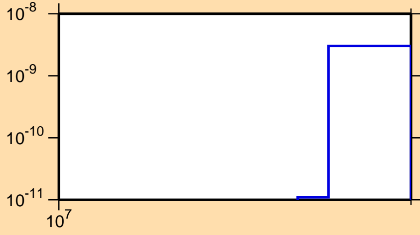
\sigma vs. E for ^{203}\text{Pb}(n,3n\alpha)
