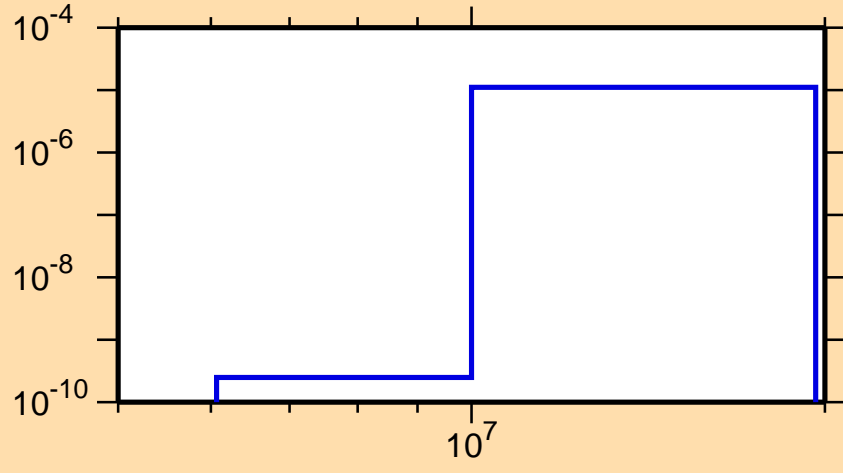
\sigma vs. E for ^{203}\text{Pb}(n,p\alpha)
