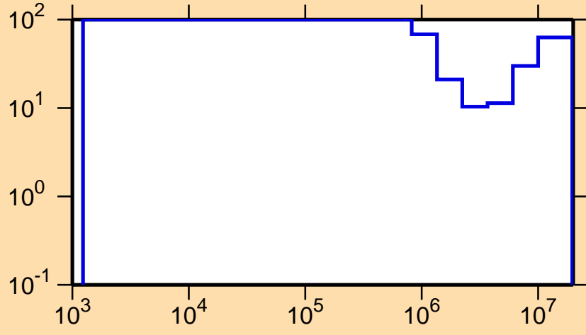
\Delta\sigma/\sigma vs. E for ^{203}\text{Pb}(n,n\text{cont.})
