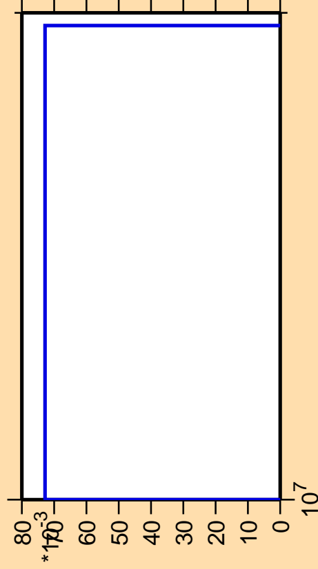
\Delta\sigma/\sigma vs. E for ^{203}\text{Pb} (mt 34)
