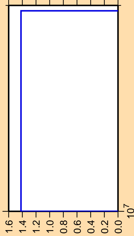
\Delta\sigma/\sigma vs. E for ^{203}\text{Pb}(\text{mt117})
