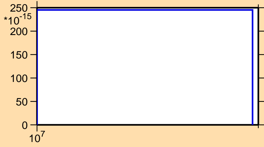
\sigma vs. E for ^{203}\text{Pb}(\text{mt117})
