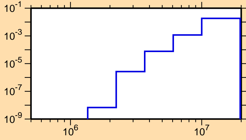
\sigma vs. E for ^{203}\text{Pb}(n,p)
