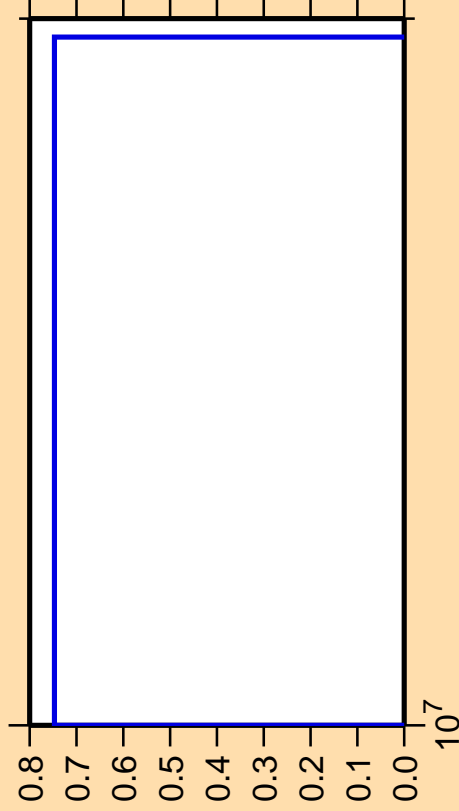
\Delta\sigma/\sigma vs. E for ^{203}\text{Pb} (mt 45)
