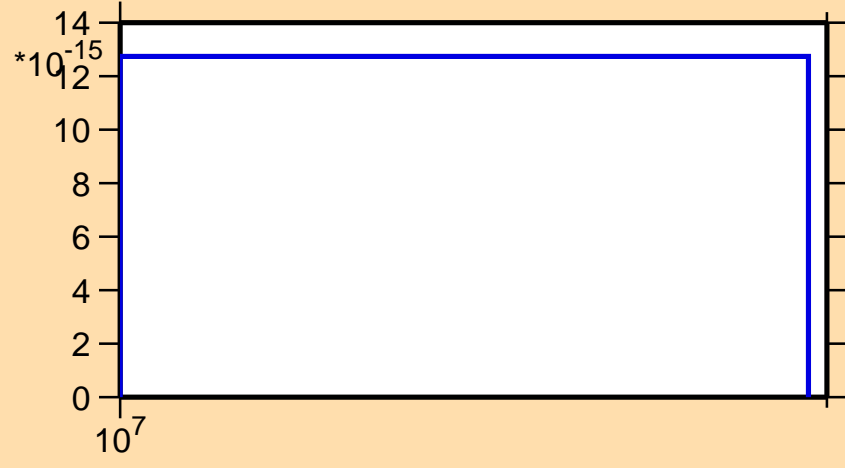
\sigma vs. E for ^{203}\text{Pb} (mt 34)
