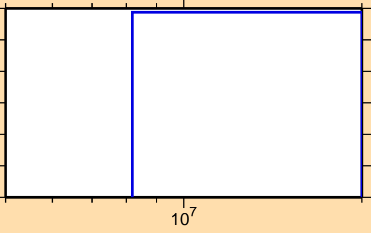
\sigma vs. E for ^{203}\text{Pb}(n,\text{nd})
