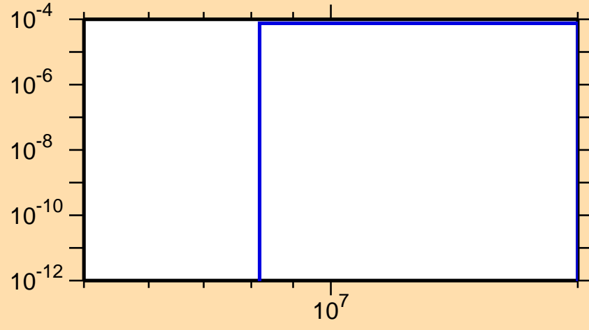
\sigma vs. E for ^{203}\text{Pb}(n,2n\alpha)
