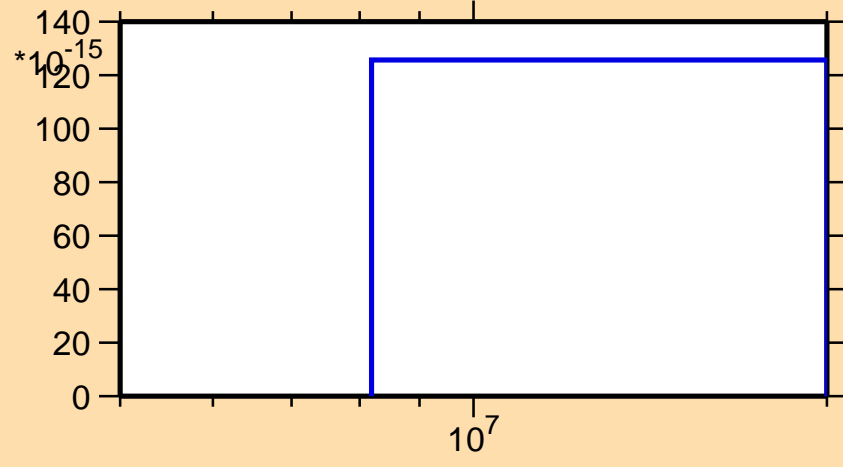
\sigma vs. E for ^{203}\text{Pb} (mt 45)
