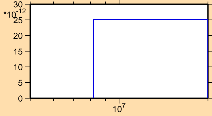
\sigma vs. E for ^{203}\text{Pb}(n,3n\alpha)
