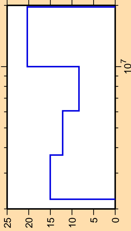
\Delta\sigma/\sigma vs. E for ^{204}\text{Pb}(n,n\text{cont.})
