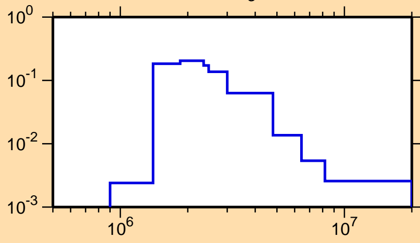
\sigma vs. E for ^{204}\text{Pb}(n,n_3)
