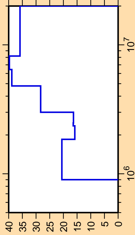
\Delta\sigma/\sigma vs. E for ^{204}\text{Pb}(n,n_3)
