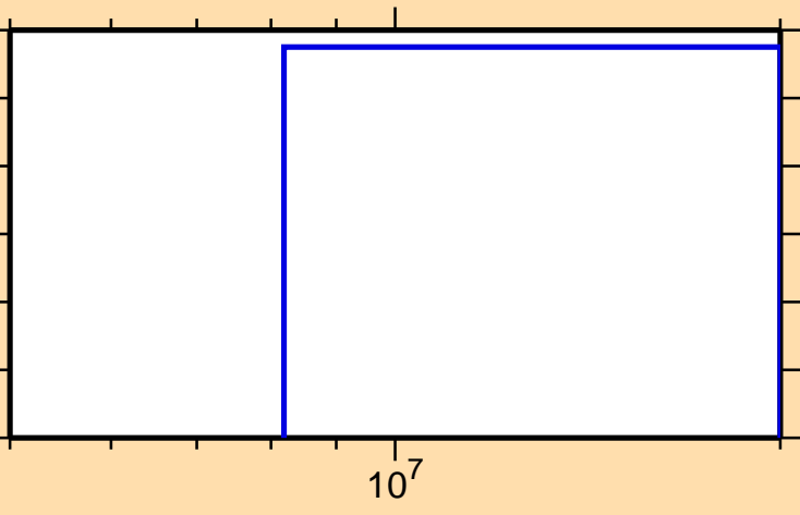
\sigma vs. E for ^{204}\text{Pb}(n,3n\alpha)
