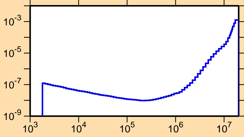
\sigma vs. E for ^{205}\text{Pb}(n,\alpha)
