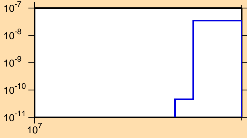
\sigma vs. E for ^{205}\text{Pb}(n,2np)
