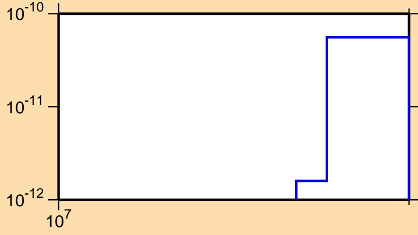
\sigma vs. E for ^{205}\text{Pb}(n,\text{He}3)
