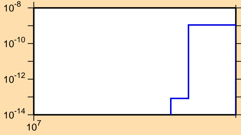
\sigma vs. E for ^{205}\text{Pb}(n,nt)
