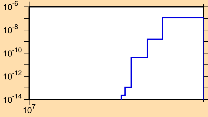
\sigma vs. E for ^{205}\text{Pb}(n,\text{nd})
