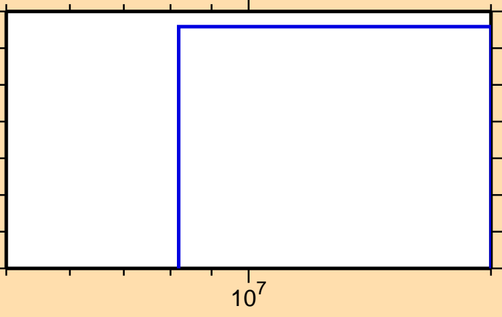
\sigma vs. E for ^{205}\text{Pb}(n,2n\alpha)
