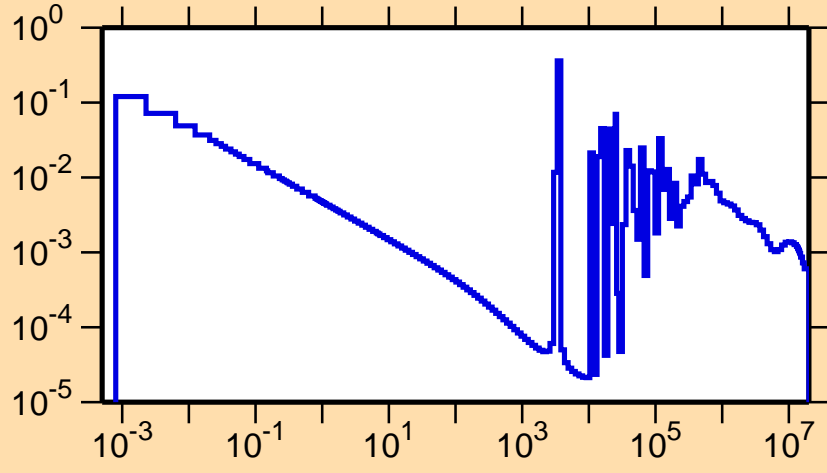
\sigma vs. E for ^{206}\text{Pb}(n,\gamma)
