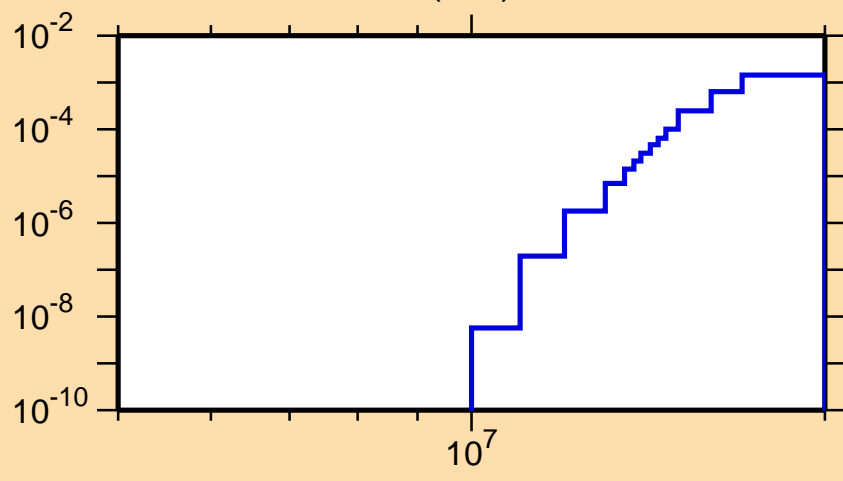
\sigma vs. E for ^{206}\text{Pb}(n,d)
