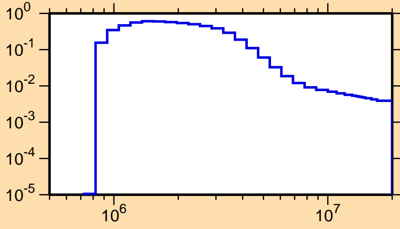
\sigma vs. E for ^{206}\text{Pb}(n,n_1)
