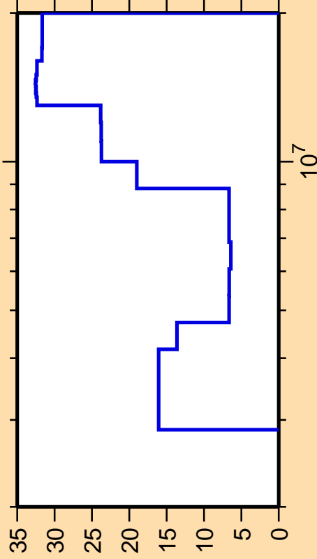
\Delta\sigma/\sigma vs. E for ^{206}\text{Pb}(n,n_{\text{cont}}) .
