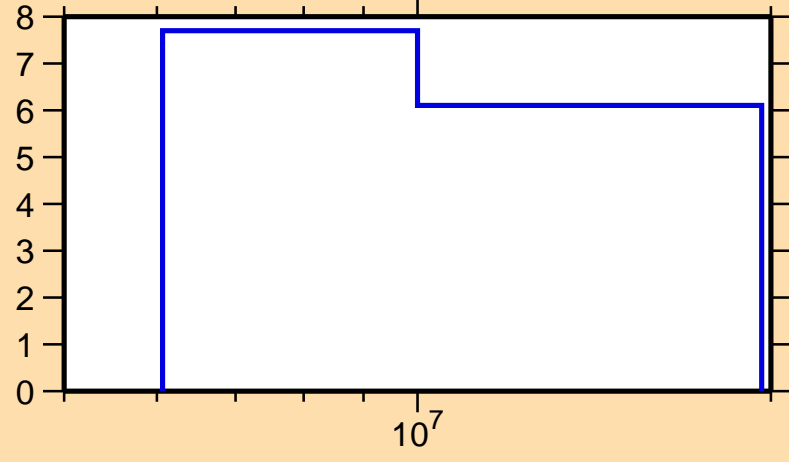
\Delta\sigma/\sigma vs. E for ^{206}\text{Pb}(n,2n)
