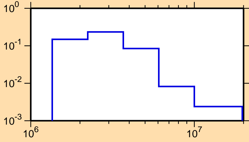
\sigma vs. E for ^{206}\text{Pb}(n,n_4)
