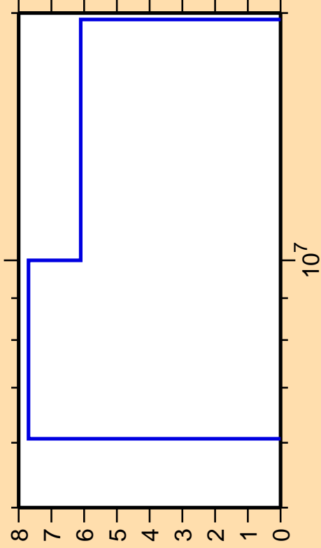
\Delta\sigma/\sigma vs. E for ^{206}\text{Pb}(n,2n)
