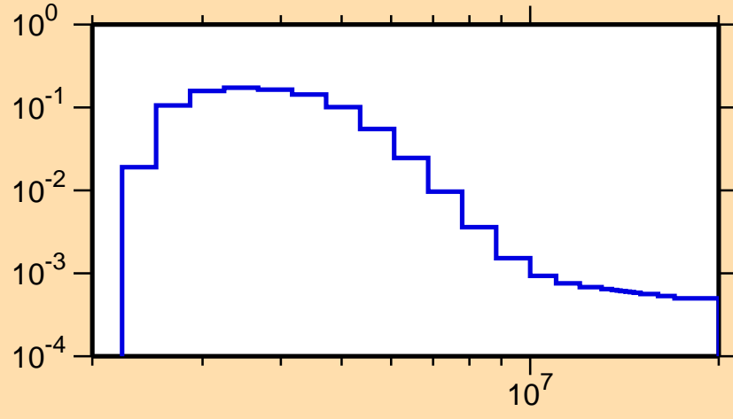
\sigma vs. E for ^{207}\text{Pb}(n,n_4)
