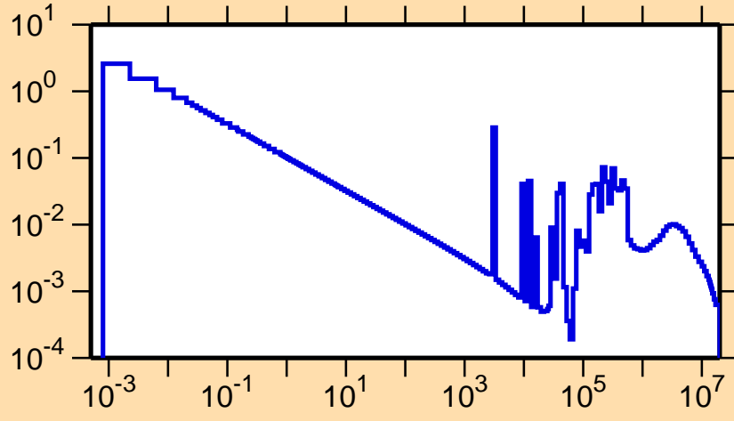
\sigma vs. E for ^{207}\text{Pb}(n,\gamma)
