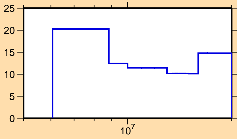
\Delta\sigma/\sigma vs. E for ^{207}\text{Pb}(n,2n)
