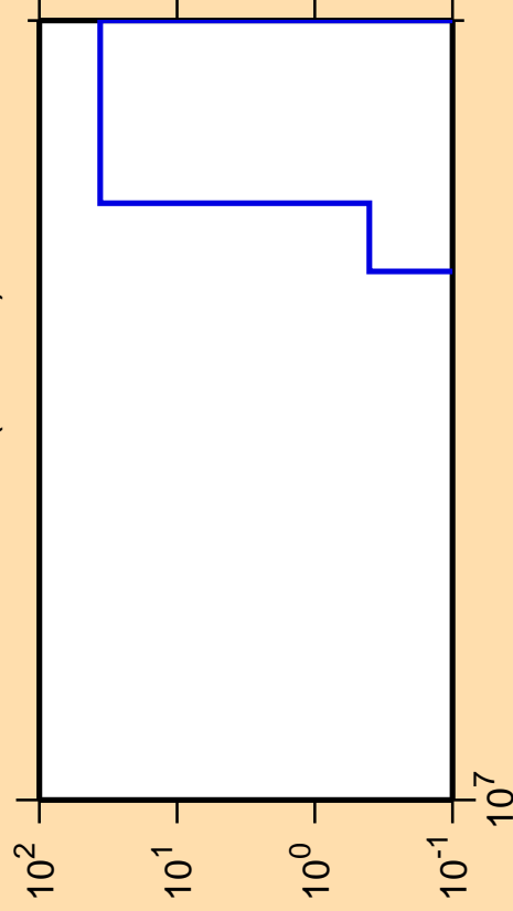
\Delta\sigma/\sigma vs. E for ^{207}\text{Pb}(n,\text{He}3)
