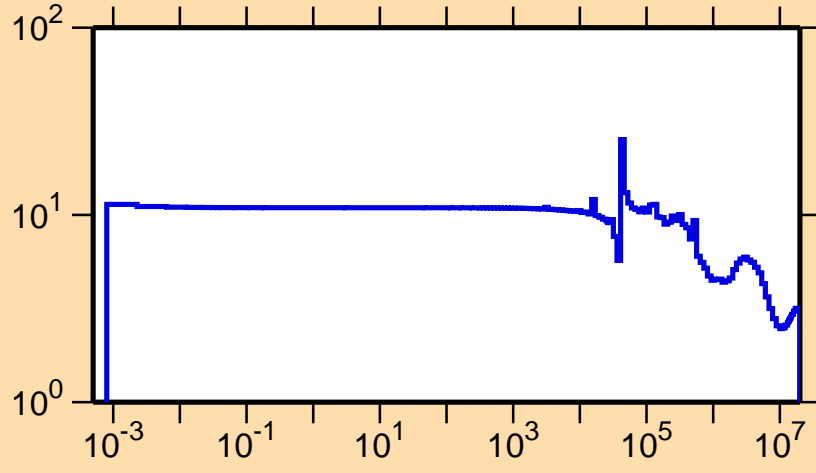
\sigma vs. E for ^{207}\text{Pb}(n,\text{el.})
