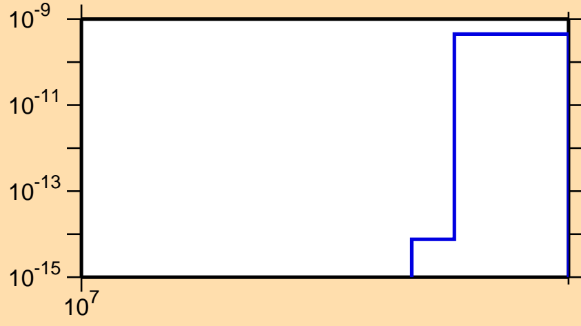
\sigma vs. E for ^{207}\text{Pb}(n,nt)
