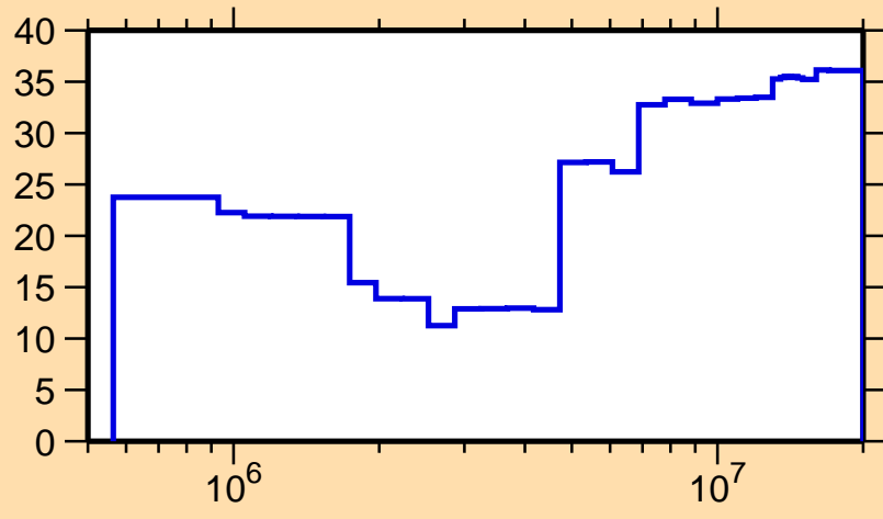
\Delta\sigma/\sigma vs. E for ^{207}\text{Pb}(n,n_1)
