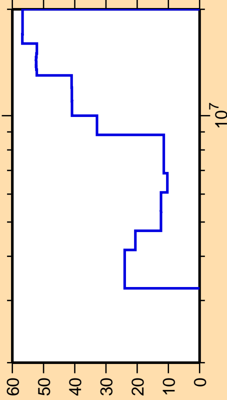
\Delta\sigma/\sigma vs. E for ^{207}\text{Pb}(n,n\text{cont.})
