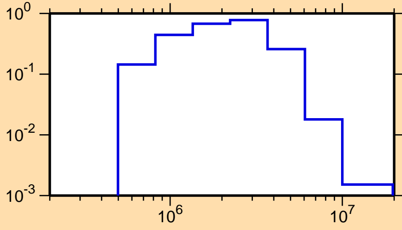
\sigma vs. E for ^{207}\text{Pb}(n,n_1)
