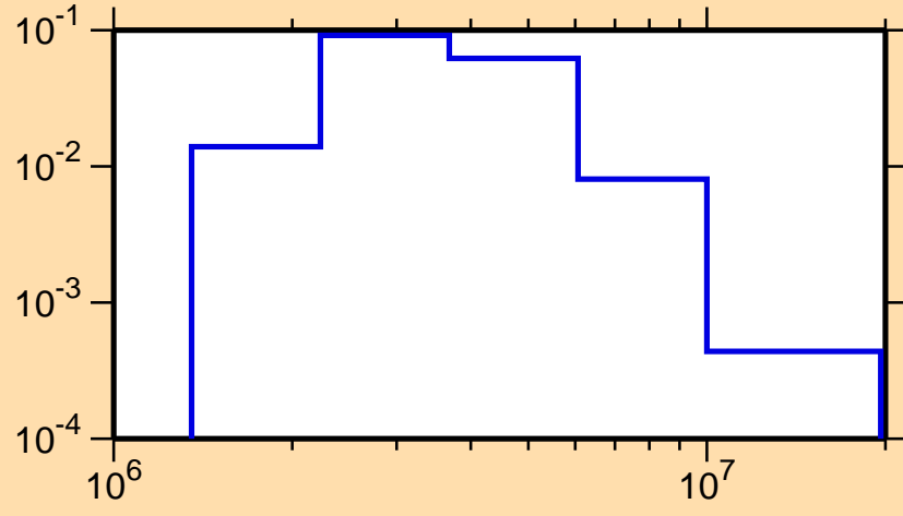
\sigma vs. E for ^{207}\text{Pb}(n,n_3)
