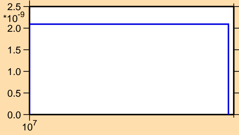
\sigma vs. E for ^{207}\text{Pb}(n,2n\alpha)
