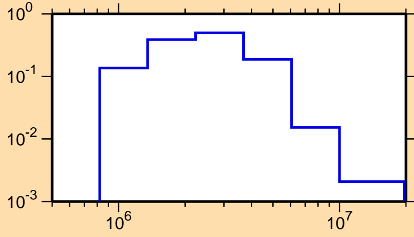
\sigma vs. E for ^{207}\text{Pb}(n,n_2)
