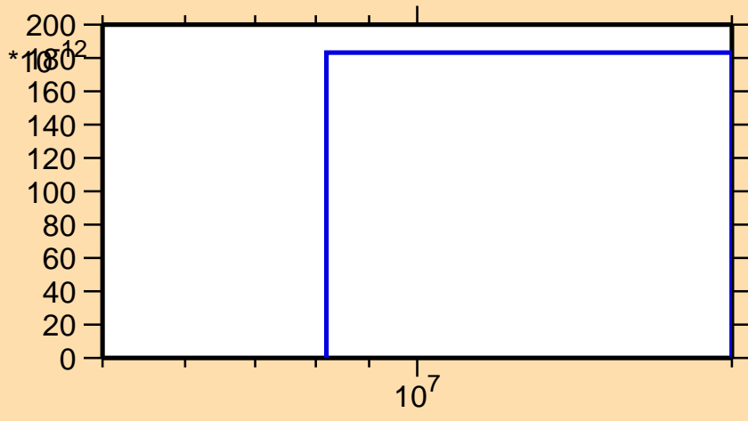
\sigma vs. E for ^{207}\text{Pb}(n,\text{nd})
