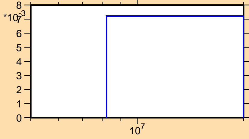
\sigma vs. E for ^{207}\text{Pb}(n,3n)
