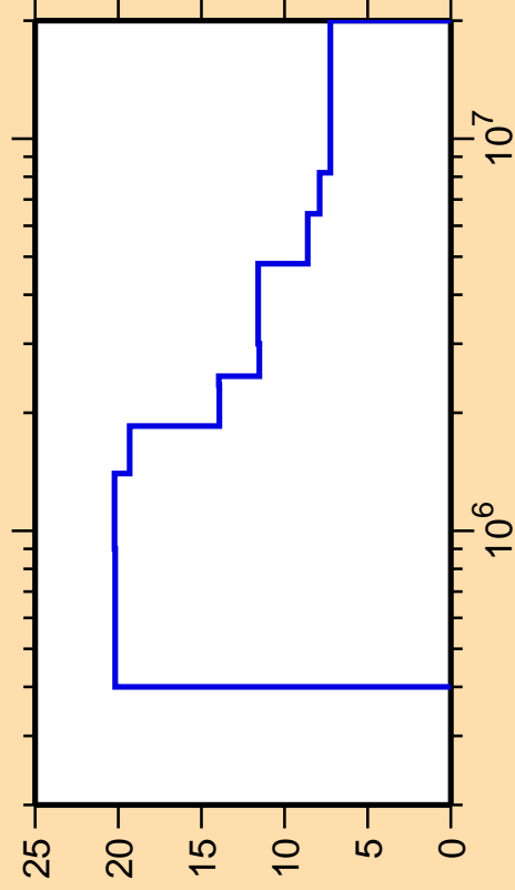
\Delta\sigma/\sigma vs. E for ^{207}\text{Pb}(n,\text{nonel.})
