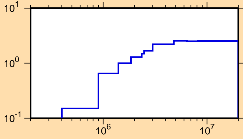
\sigma vs. E for ^{207}\text{Pb}(n,\text{nonel.})
