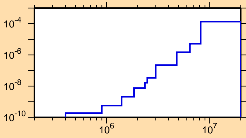
\sigma vs. E for ^{207}\text{Pb}(n,\alpha)
