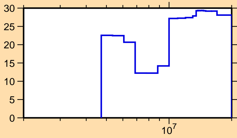
\Delta\sigma/\sigma vs. E for ^{208}\text{Pb}(n,n\text{cont.})
