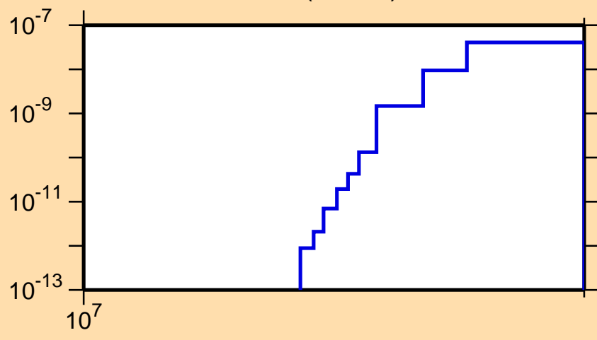
\sigma vs. E for ^{208}\text{Pb}(n,2n\alpha)
