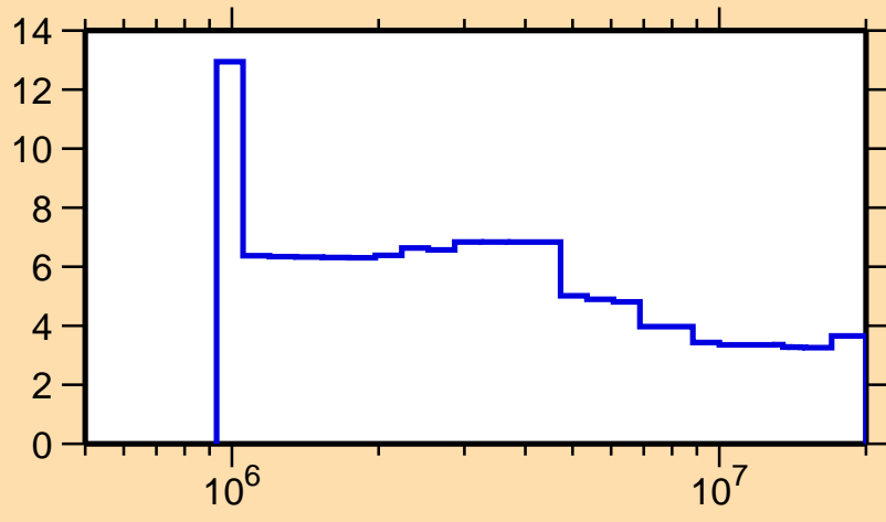
\Delta\sigma/\sigma vs. E for ^{208}\text{Pb}(n,\text{tot.})
