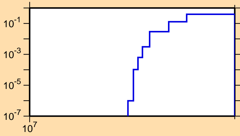
\sigma vs. E for ^{208}\text{Pb}(n,3n)
