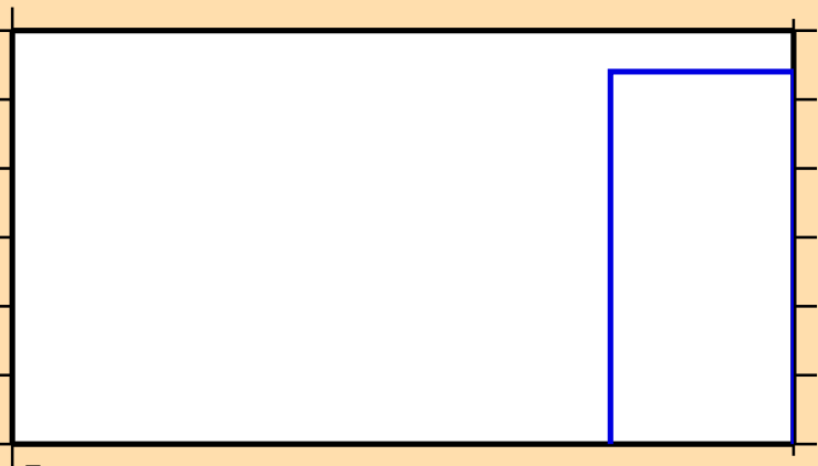
\sigma vs. E for ^{208}\text{Pb}(n,2np)
