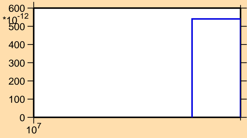
\sigma vs. E for ^{208}\text{Pb}(n,2np)
