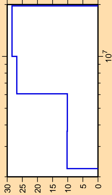
\Delta\sigma/\sigma vs. E for ^{208}\text{Pb}(n,n_2)
