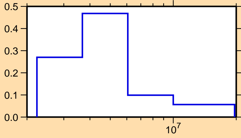
\sigma vs. E for ^{208}\text{Pb}(n,n_1)
