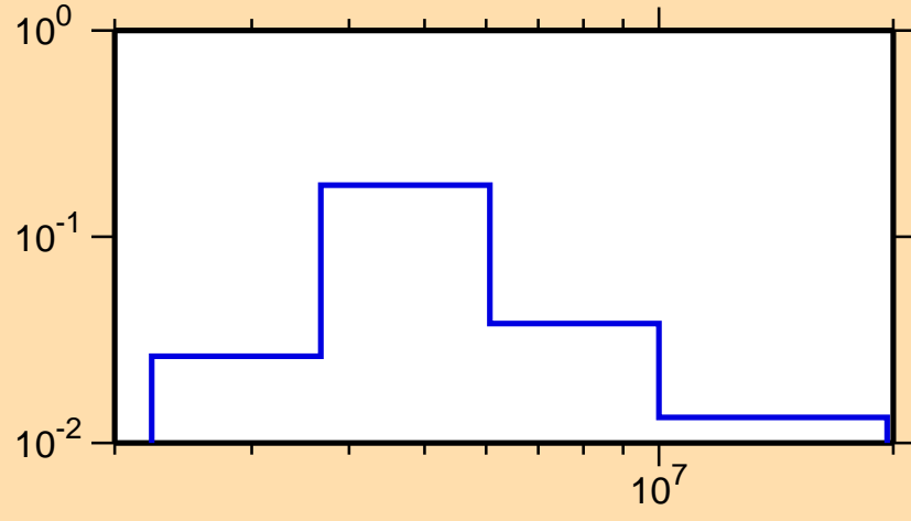
\sigma vs. E for ^{208}\text{Pb}(n,n_2)
