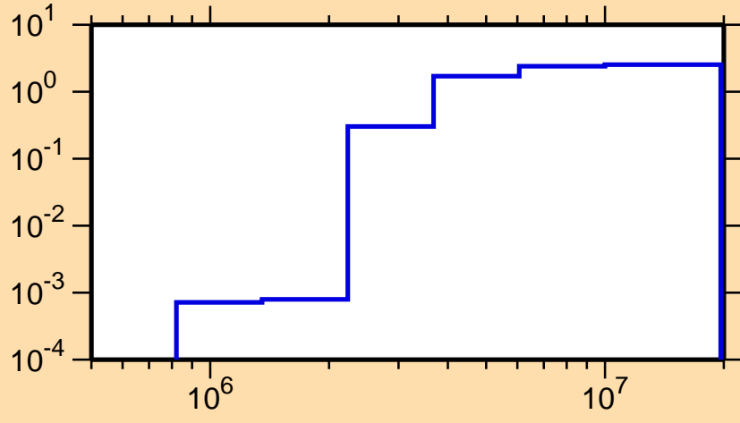
\sigma vs. E for ^{208}\text{Pb}(n,\text{nonel.})
