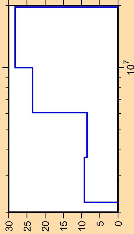
\Delta\sigma/\sigma vs. E for ^{208}\text{Pb}(n,n_1)
