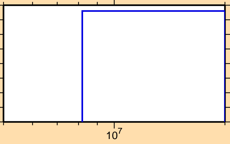
\sigma vs. E for ^{208}\text{Pb}(n,\text{He}3)
