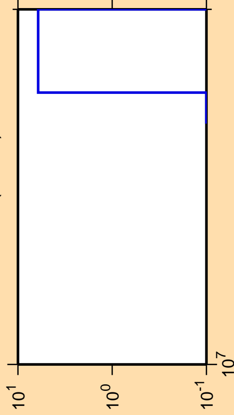
\Delta\sigma/\sigma vs. E for ^{209}\text{Pb}(n,3n\alpha)
