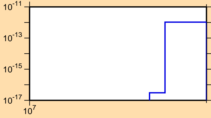
\sigma vs. E for ^{209}\text{Pb}(n,3n\alpha)
