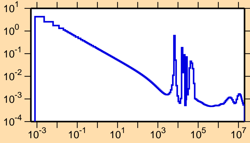
\sigma vs. E for ^{209}\text{Pb}(n,\gamma)
