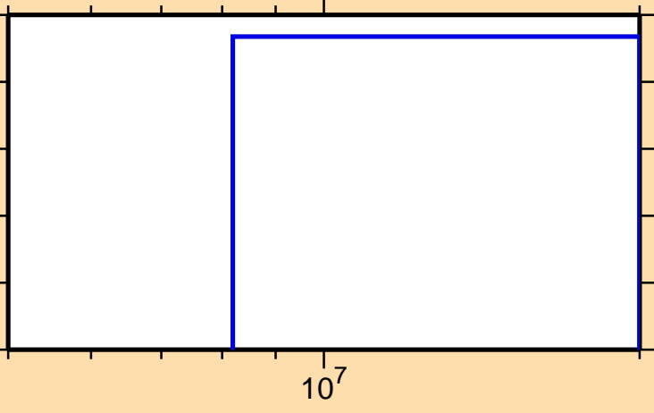
\sigma vs. E for ^{209}\text{Pb}(n,2np)
