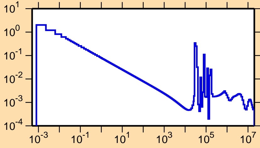
\sigma vs. E for ^{210}\text{Pb}(n,\gamma)
