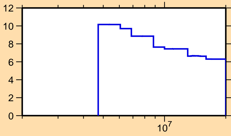
\Delta\sigma/\sigma vs. E for ^{210}\text{Pb}(n,\text{nonel.})
