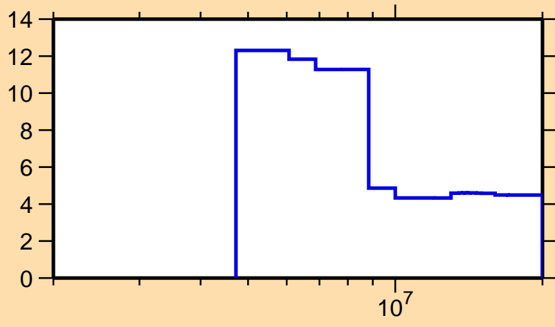
\Delta\sigma/\sigma vs. E for ^{210}\text{Pb}(n,\text{tot.})
