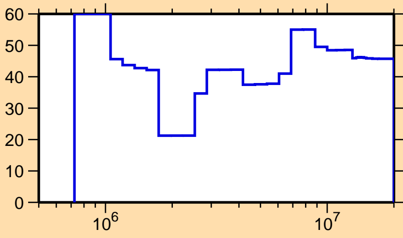
\Delta\sigma/\sigma vs. E for ^{210}\text{Pb}(n,n_1)
