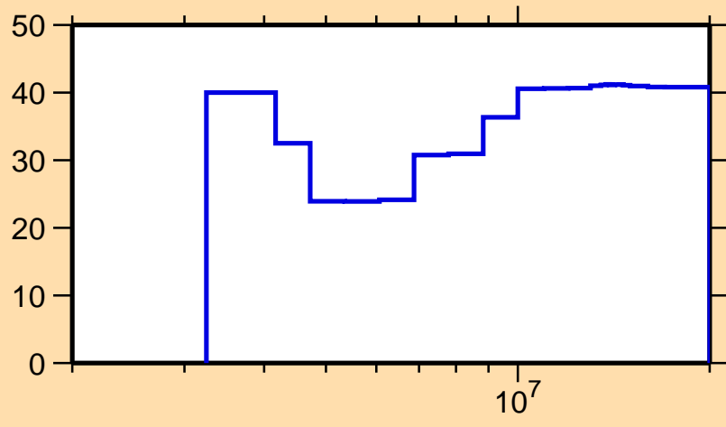
\Delta\sigma/\sigma vs. E for ^{210}\text{Pb}(n,n\text{cont.})
