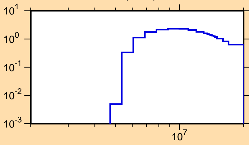
\sigma vs. E for ^{210}\text{Pb}(n,2n)
