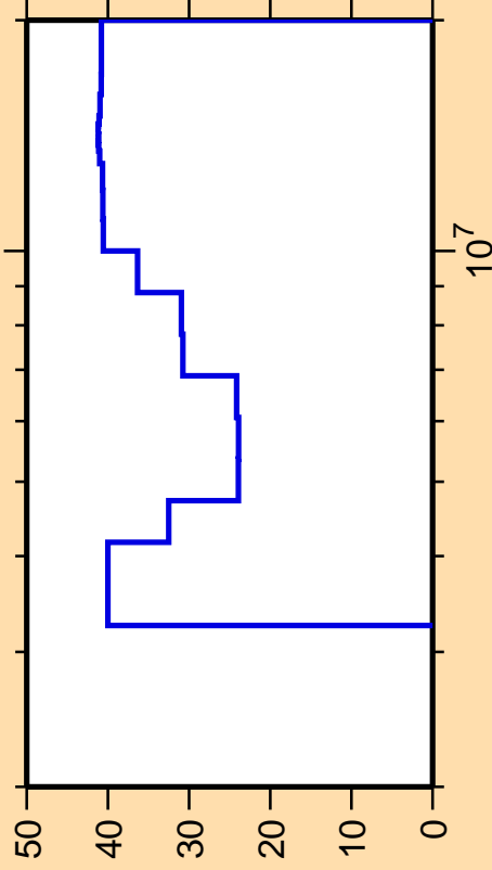
\Delta\sigma/\sigma vs. E for ^{210}\text{Pb}(n,n\text{cont.})
