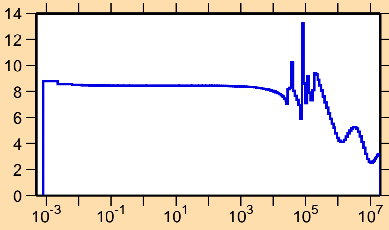
\sigma vs. E for ^{210}\text{Pb}(n,\text{el.})
