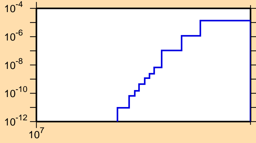
\sigma vs. E for ^{210}\text{Pb}(n,nt)
