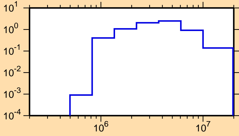
\sigma vs. E for ^{210}\text{Pb}(n,\text{inel.})
