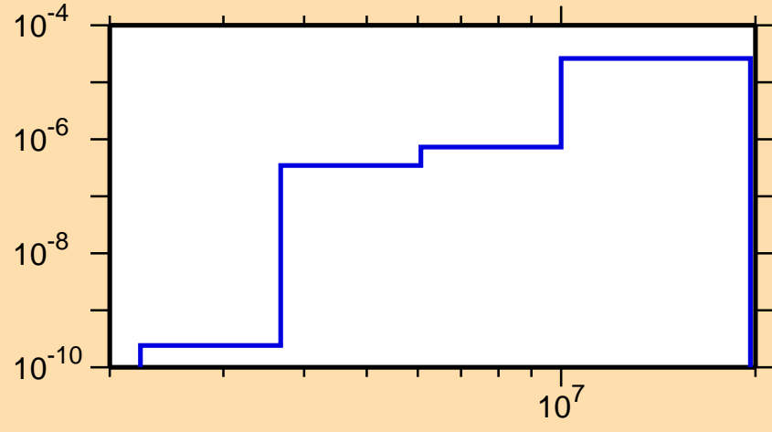
\sigma vs. E for ^{210}\text{Pb}(n,n\alpha)
