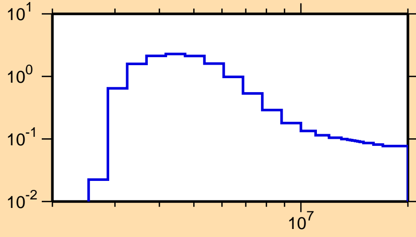
\sigma vs. E for ^{211}\text{Pb}(n,n\text{cont.})
