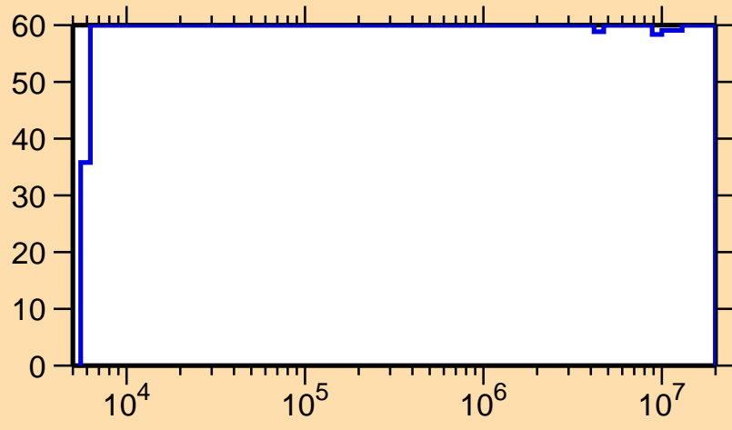
\Delta\sigma/\sigma vs. E for ^{211}\text{Pb}(n,\gamma)
