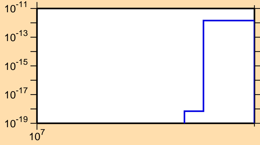
\sigma vs. E for ^{211}\text{Pb}(\text{mt117})
