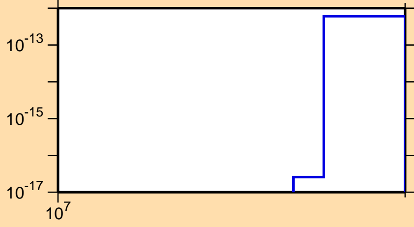
\sigma vs. E for ^{211}\text{Pb} (mt 11)
