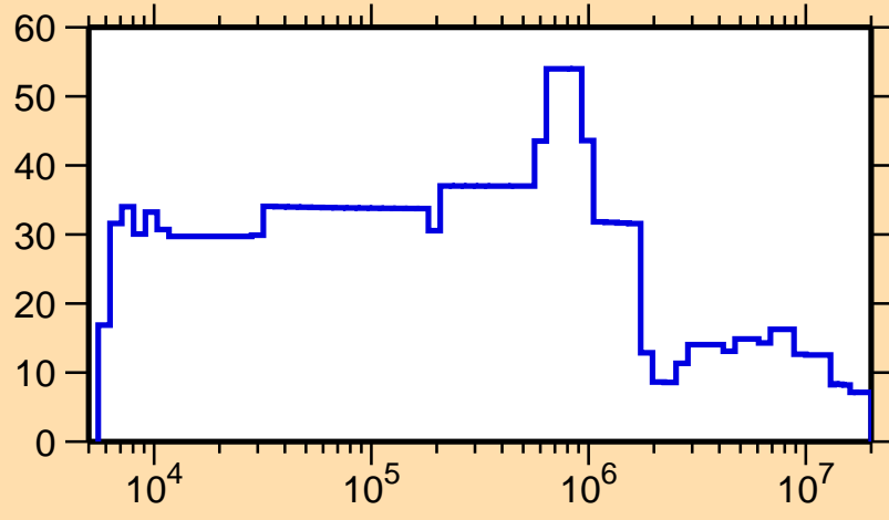
\Delta\sigma/\sigma vs. E for ^{211}\text{Pb}(n,\text{tot.})
