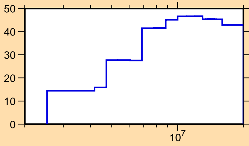
\Delta\sigma/\sigma vs. E for ^{211}\text{Pb}(n,n\text{cont.})
