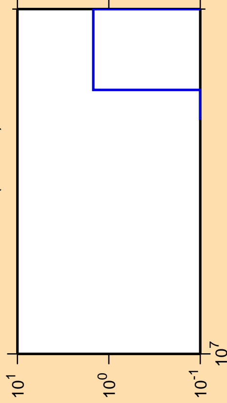
\Delta\sigma/\sigma vs. E for ^{211}\text{Pb}(\text{mt117})
