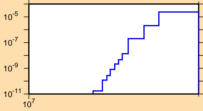
\sigma vs. E for ^{211}\text{Pb}(n,nt)
