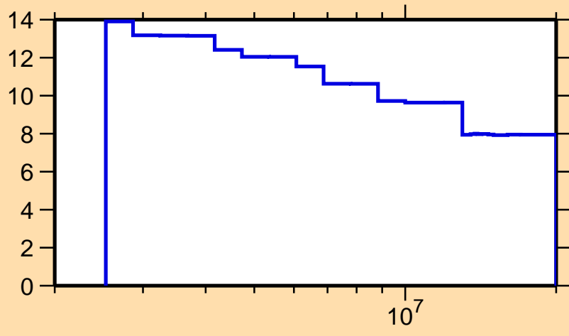
\Delta\sigma/\sigma vs. E for ^{211}\text{Pb}(n,\text{nonel.})
