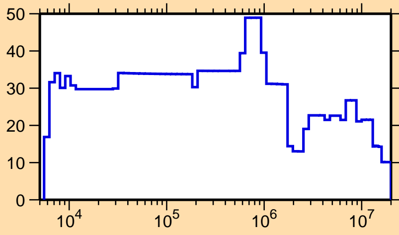
\Delta\sigma/\sigma vs. E for ^{211}\text{Pb}(n,\text{el.})
