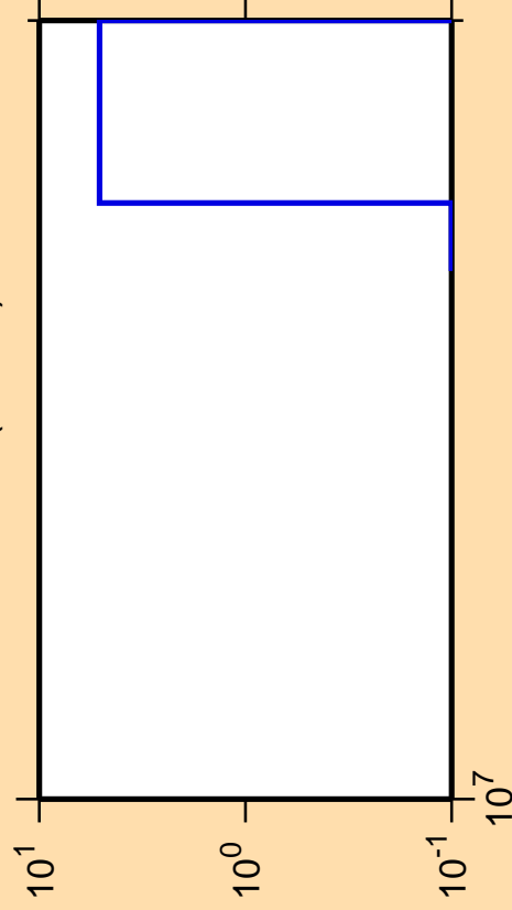
\Delta\sigma/\sigma vs. E for ^{211}\text{Pb} (mt 11)
