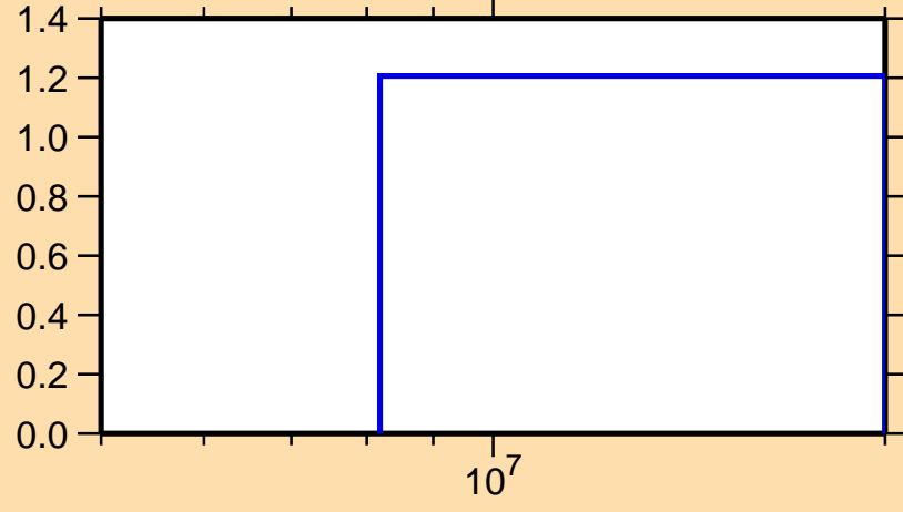
\sigma vs. E for ^{211}\text{Pb}(n,3n)
