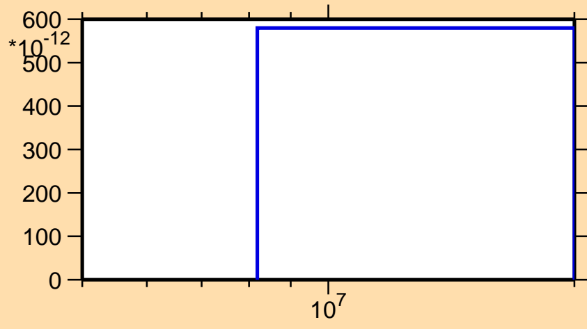
\sigma vs. E for ^{211}\text{Pb}(n,3n\alpha)
