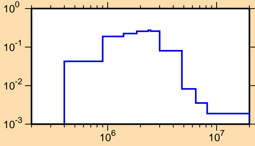
\sigma vs. E for ^{211}\text{Pb}(n,n_4)
