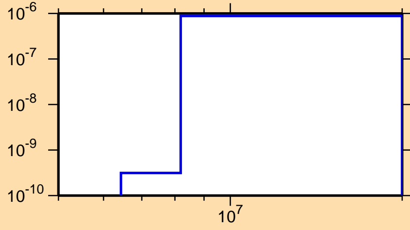
\sigma vs. E for ^{211}\text{Pb}(n,2n\alpha)
