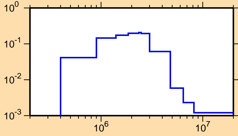
\sigma vs. E for ^{211}\text{Pb}(n,n_2)
