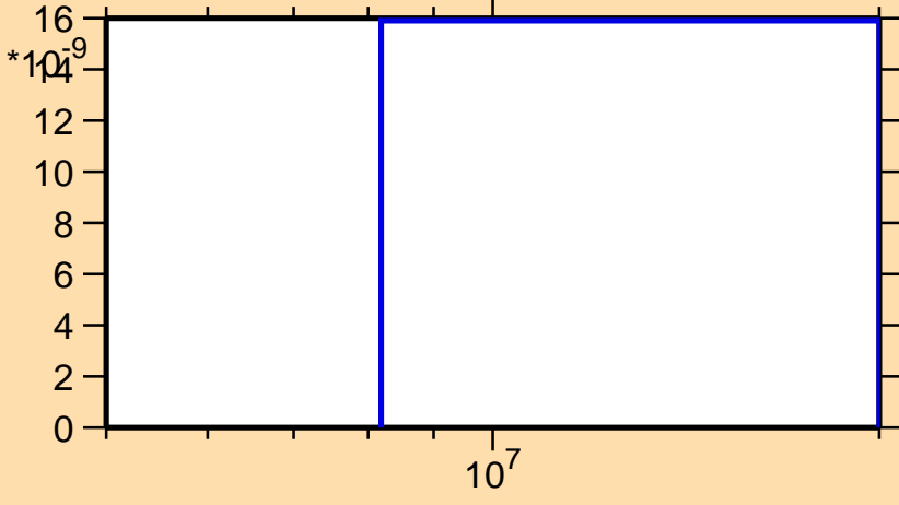
\sigma vs. E for ^{211}\text{Pb}(n,\text{nd})
