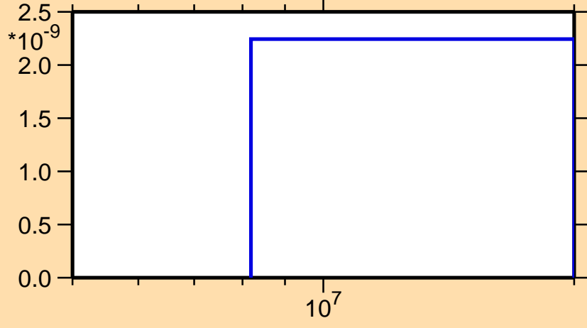
\sigma vs. E for ^{211}\text{Pb}(n,p\alpha)
