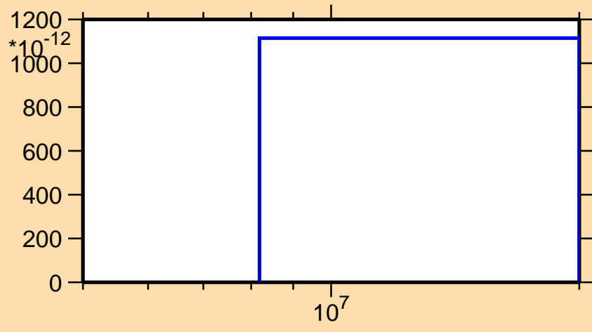
\sigma vs. E for ^{211}\text{Pb}(n,2np)
