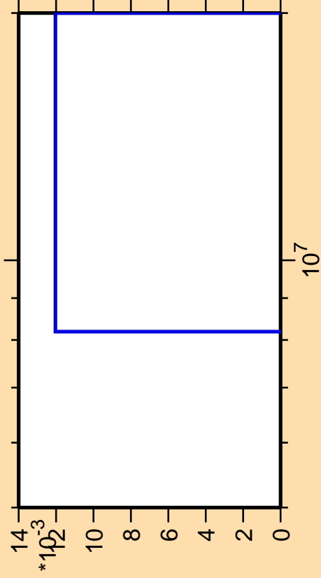
\Delta\sigma/\sigma vs. E for ^{211}\text{Pb}(\text{mt117})
