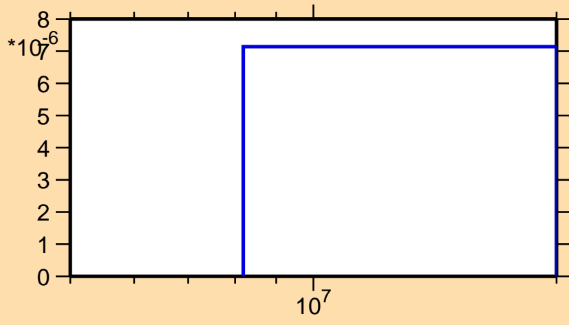
\sigma vs. E for ^{211}\text{Pb}(n,np)
