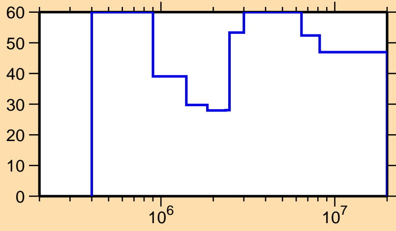
\Delta\sigma/\sigma vs. E for ^{211}\text{Pb}(n,n_1)
