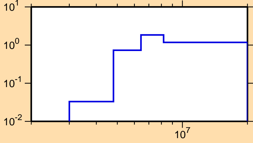
\sigma vs. E for ^{211}\text{Pb}(n,2n)
