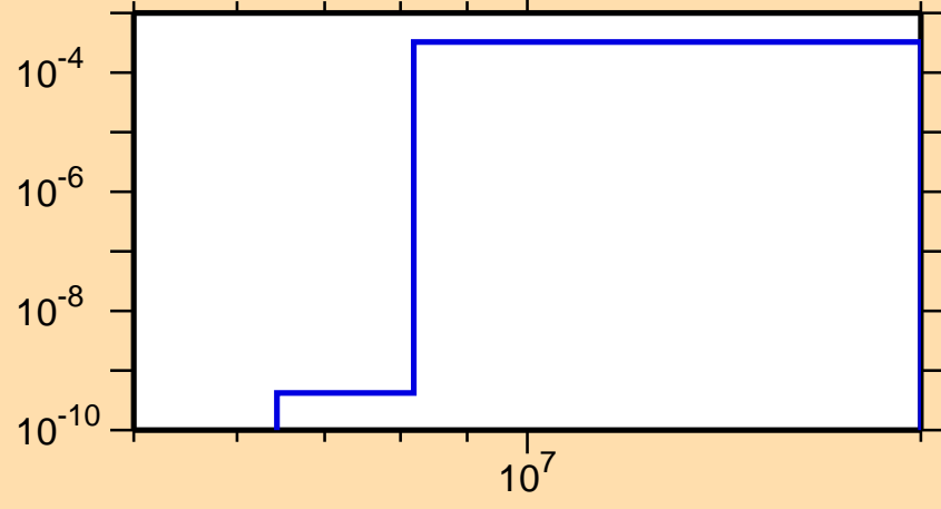
\sigma vs. E for ^{211}\text{Pb}(n,p)
