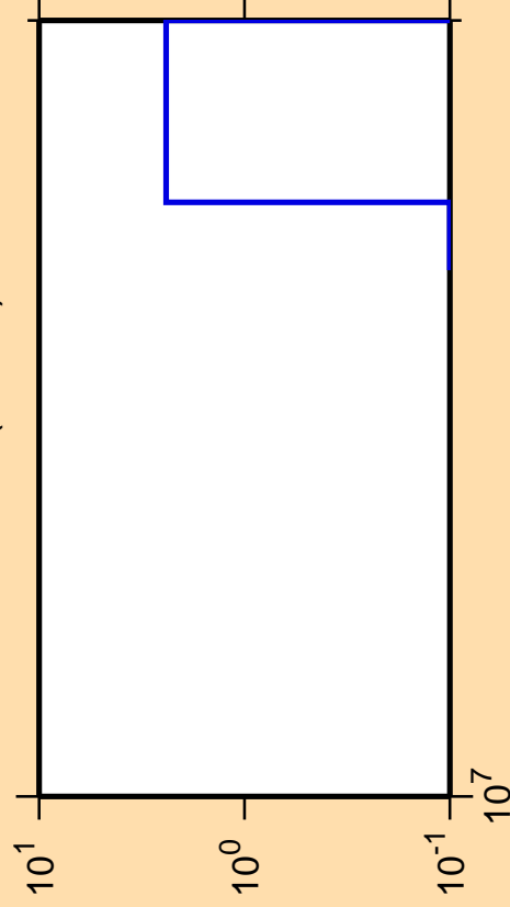
\Delta\sigma/\sigma vs. E for ^{212}\text{Pb} (mt 45)
