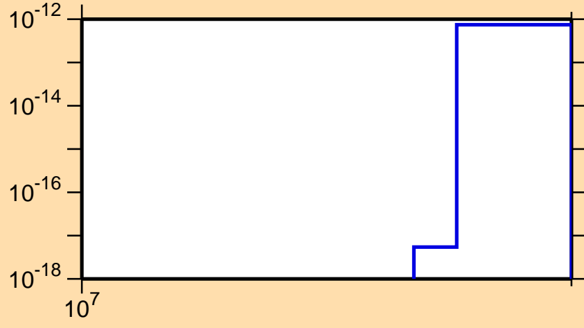
\sigma vs. E for ^{212}\text{Pb} (mt 45)
