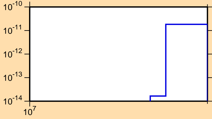
\sigma vs. E for ^{212}\text{Pb}(\text{mt117})
