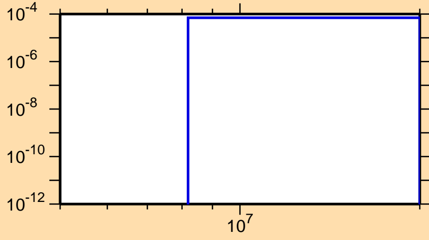
\sigma vs. E for ^{212}\text{Pb}(n,p)
