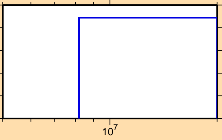
\sigma vs. E for ^{212}\text{Pb}(n,3n\alpha)
