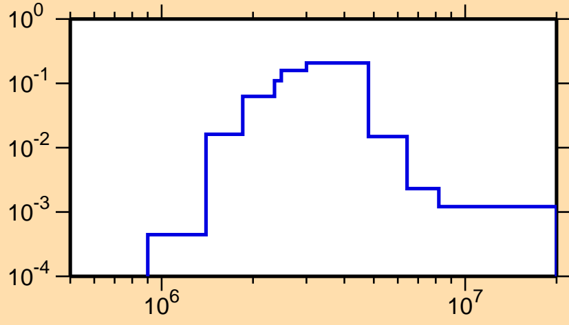
\sigma vs. E for ^{212}\text{Pb}(n,n_3)
