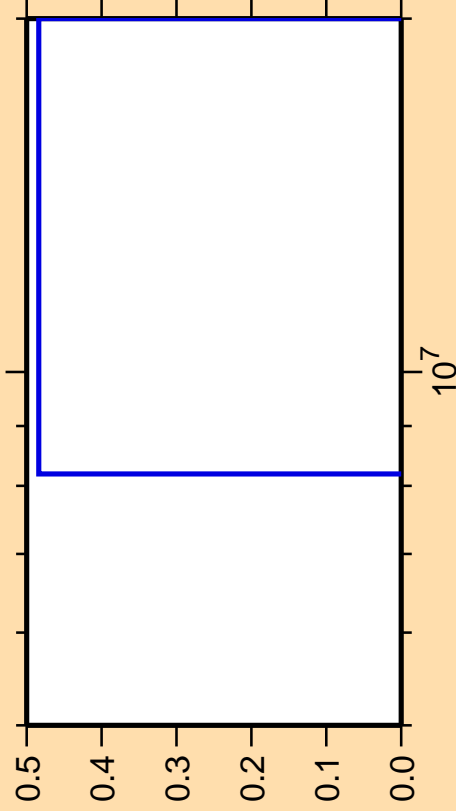
\Delta\sigma/\sigma vs. E for ^{212}\text{Pb}(\text{mt117})
