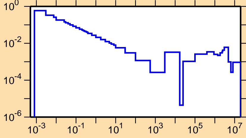
\sigma vs. E for ^{212}\text{Pb}(n,\gamma)
