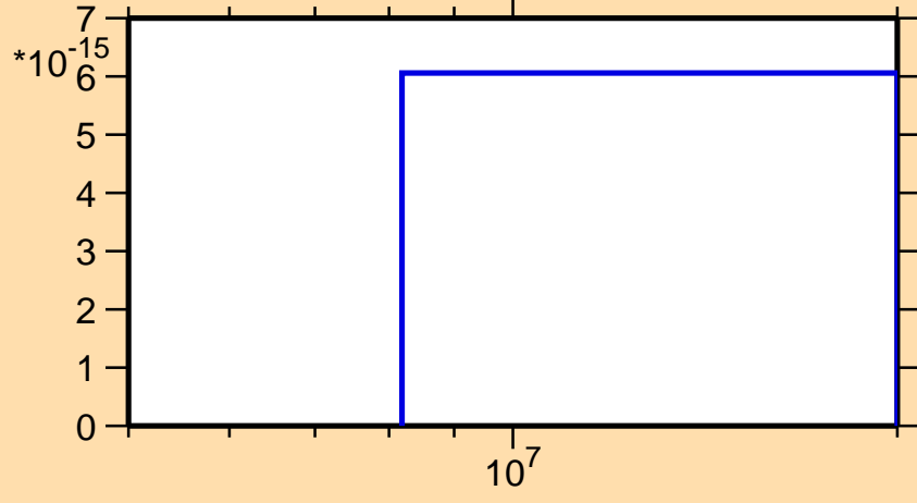
\sigma vs. E for ^{212}\text{Pb} (mt 45)
