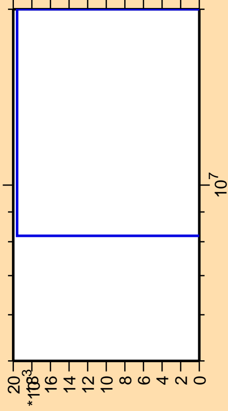
\Delta\sigma/\sigma vs. E for ^{212}\text{Pb} (mt 45)
