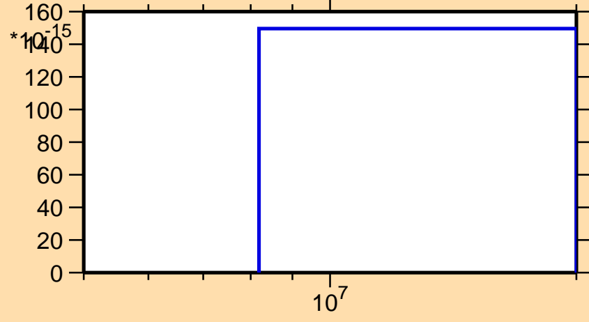
\sigma vs. E for ^{212}\text{Pb}(\text{mt117})
