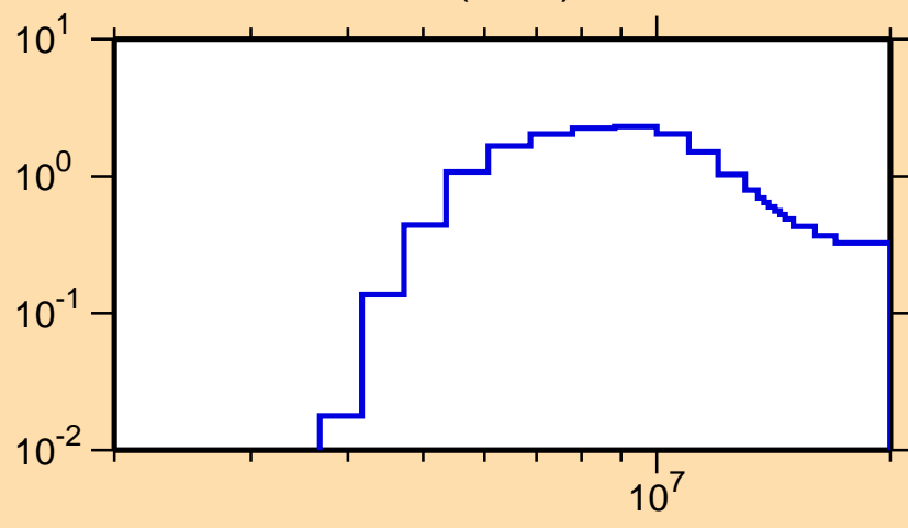
\sigma vs. E for ^{213}\text{Pb}(n,2n)
